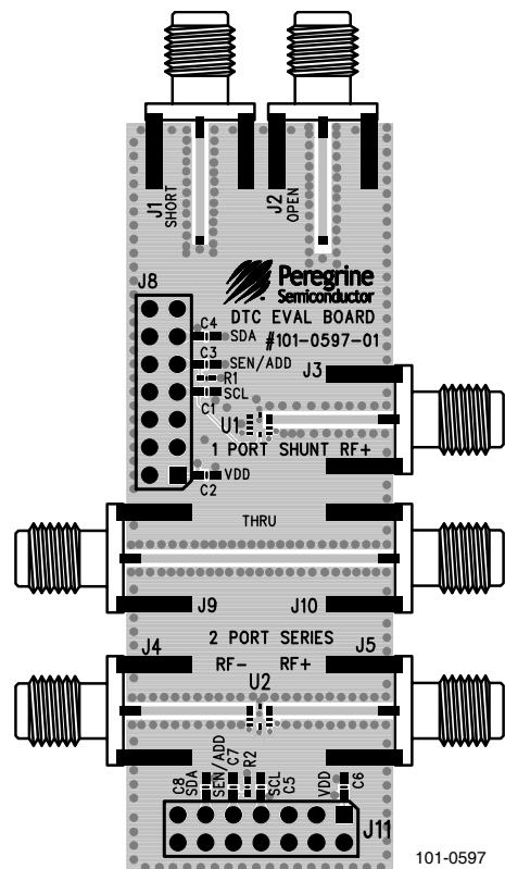
Figure 21. Evaluation Board
