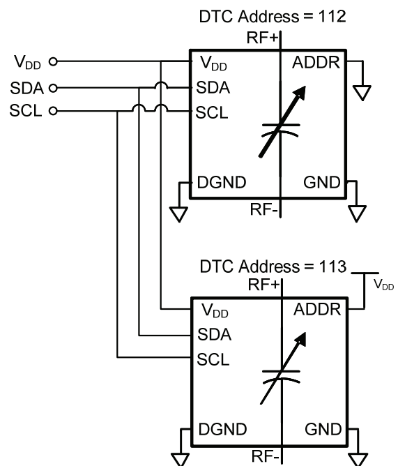
Figure 17. Recommended Bus Sharing
