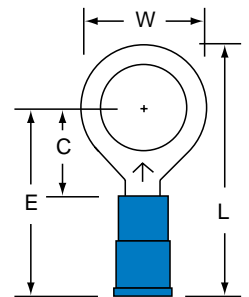
MNG14-38R Stud Size 3/8 Wire Range 16-14
