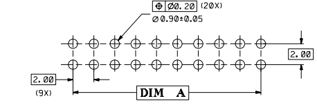
RECOMMENDED PCB PATTERN
