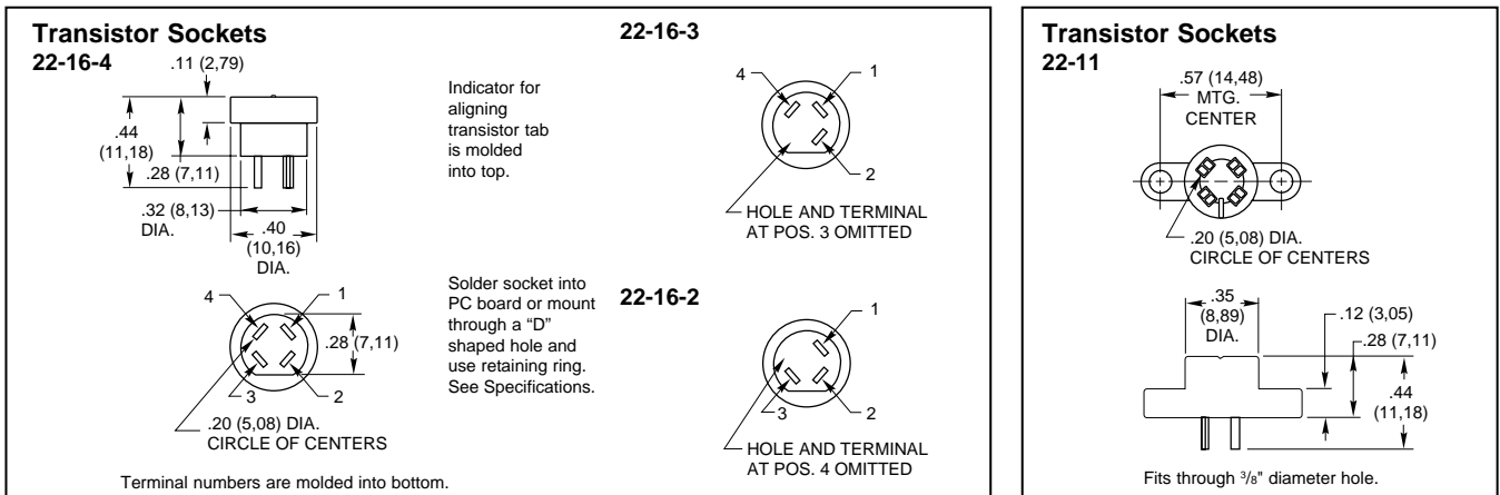
Transistor Sockets
