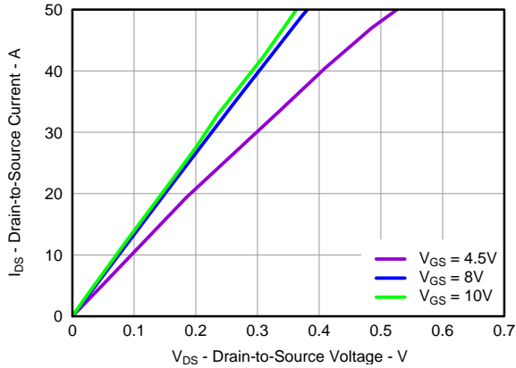
Figure 3. Saturation Characteristics
