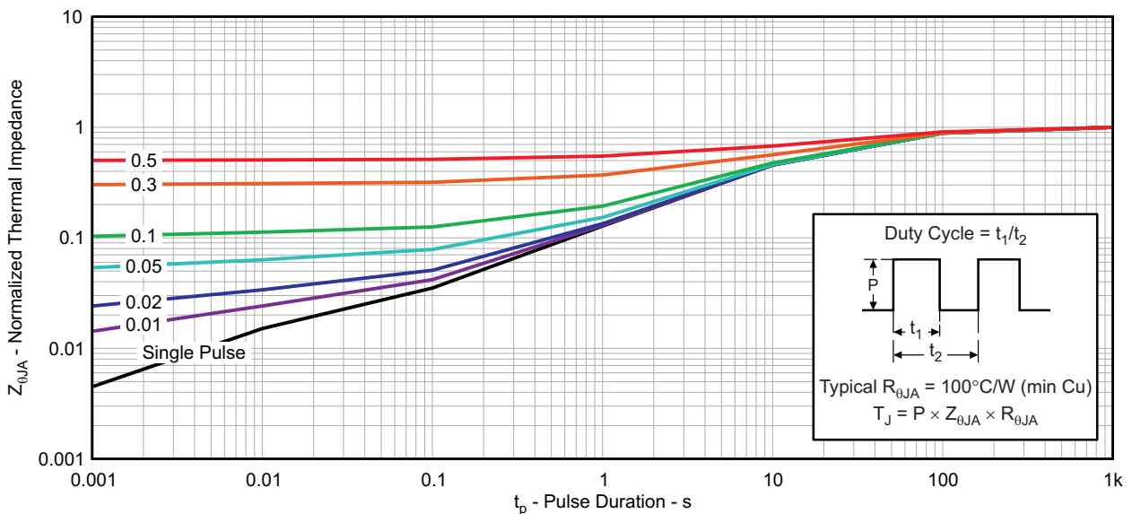
Figure 2. Transient Thermal Impedance
