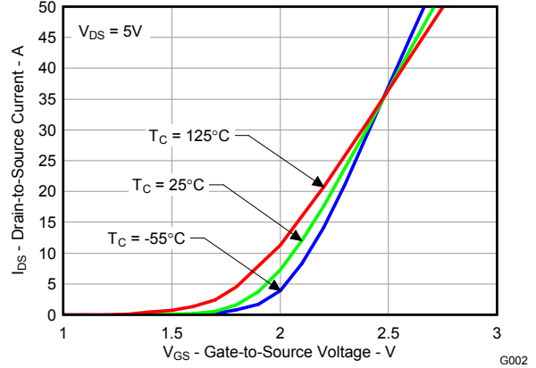
Figure 4. Transfer Characteristics
