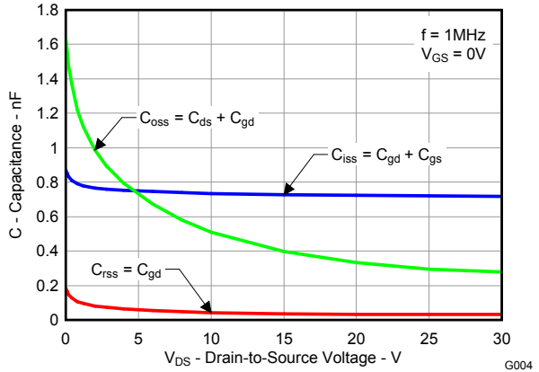
Figure 6. Capacitance
