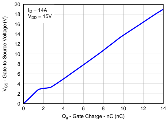
Figure 5. Gate Charge
