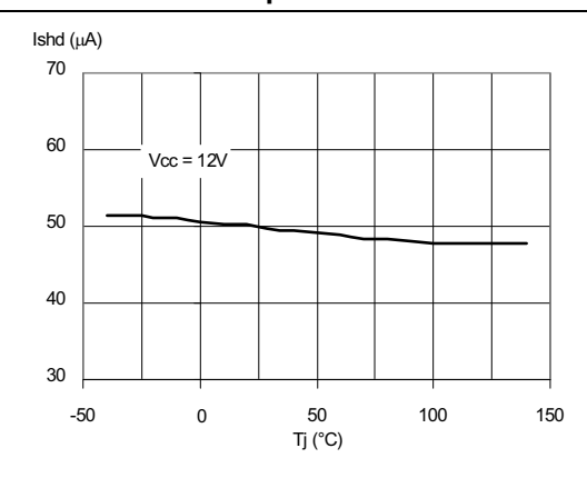
Figure 34. Shutdown current vs. junction temperature
