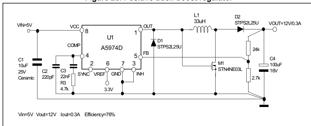
Figure 26. Positive buck-boost regulator
