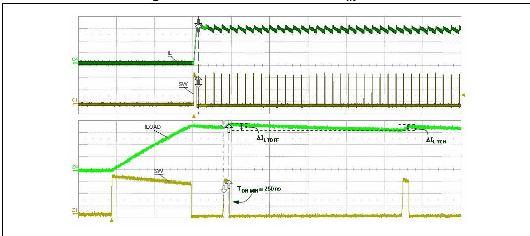
Figure 19. Short-circuit current V_{IN} = 12\text{ V}
