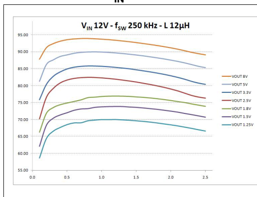
Figure 40. Efficiency vs. output current V_{IN} = 12\text{ V}
