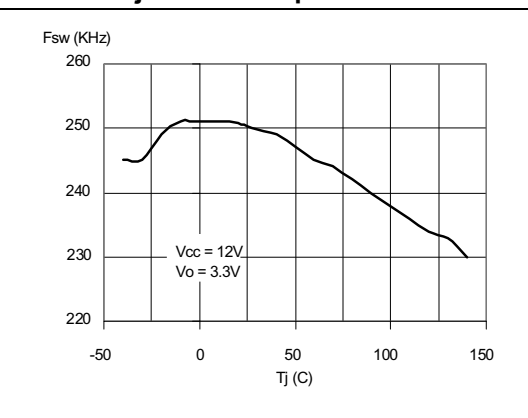
Figure 36. Switching frequency vs. junction temperature
