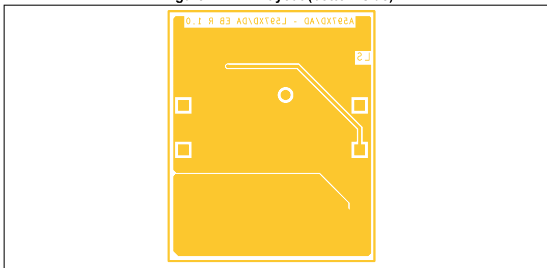
Figure 24. PCB layout (bottom side)
