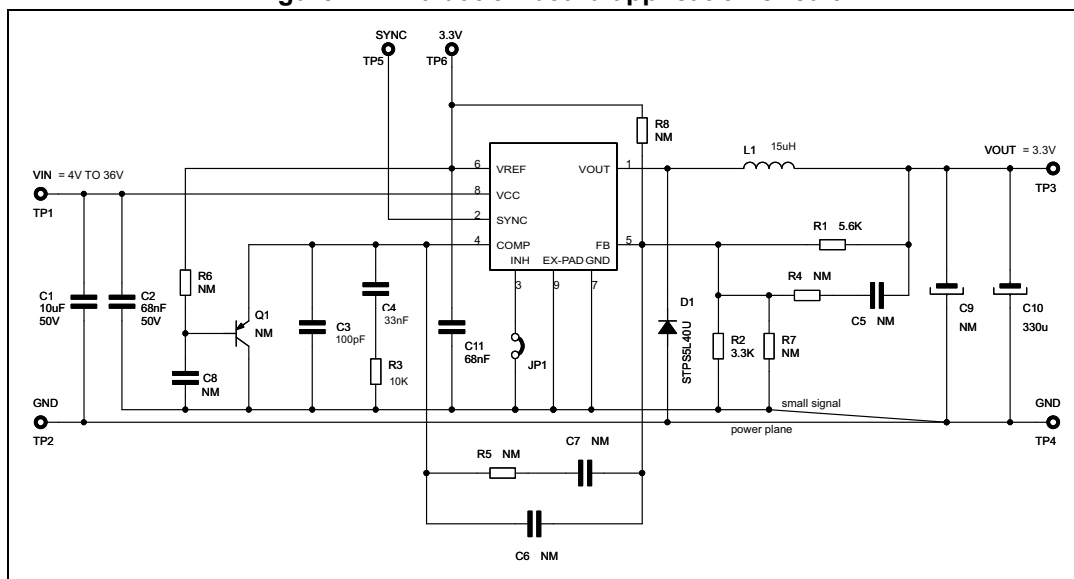
Figure 22. Evaluation board application circuit
