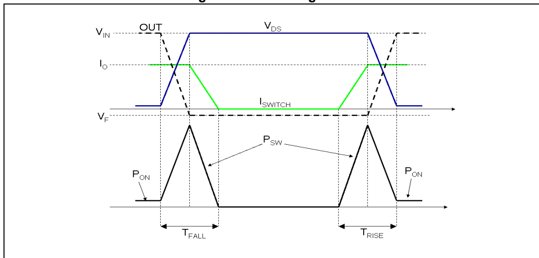
Figure 14. Switching losses
