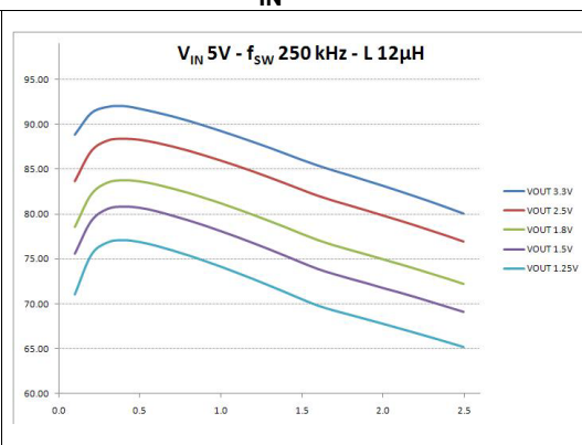
Figure 41. Efficiency vs. output current V_{IN} = 5\text{ V}
