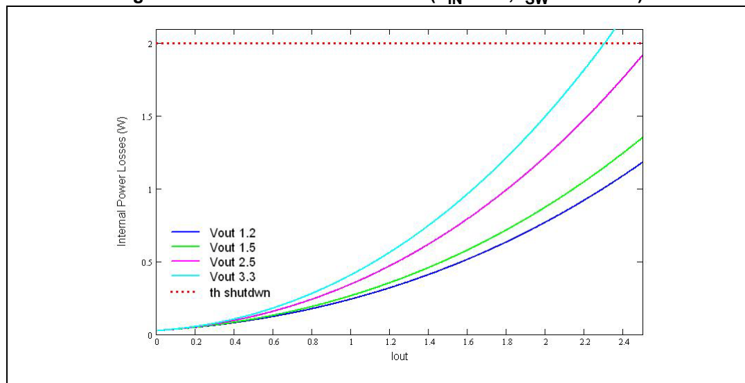
Figure 15. Power losses estimation ( V_{IN} = 5\text{ V} , f_{SW} = 250\text{ kHz} )
