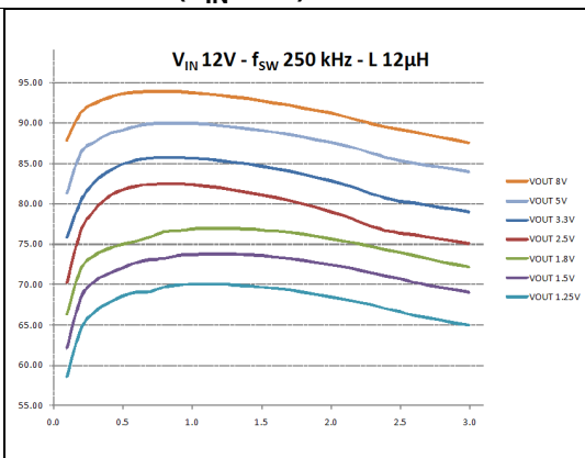
Figure 40. Efficiency vs. output current ( V_{IN} 12 V)
