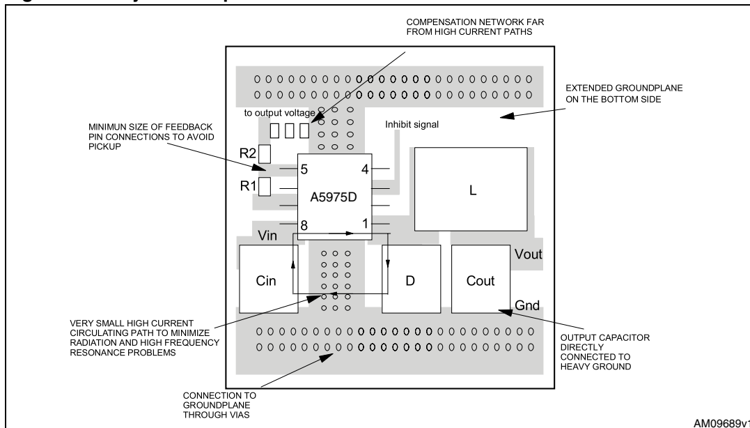
Figure 13. Layout example
