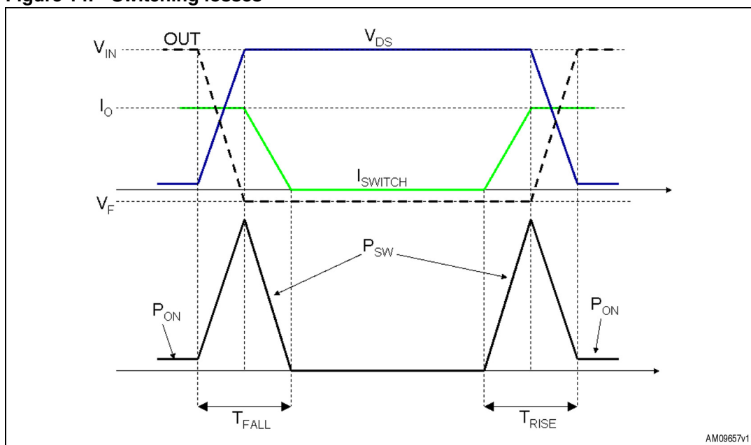
Figure 14. Switching losses
