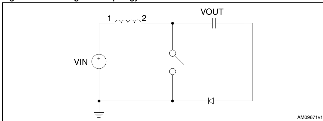
Figure 28. Floating boost topology
