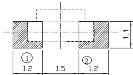
Recommend Soldering Pad
