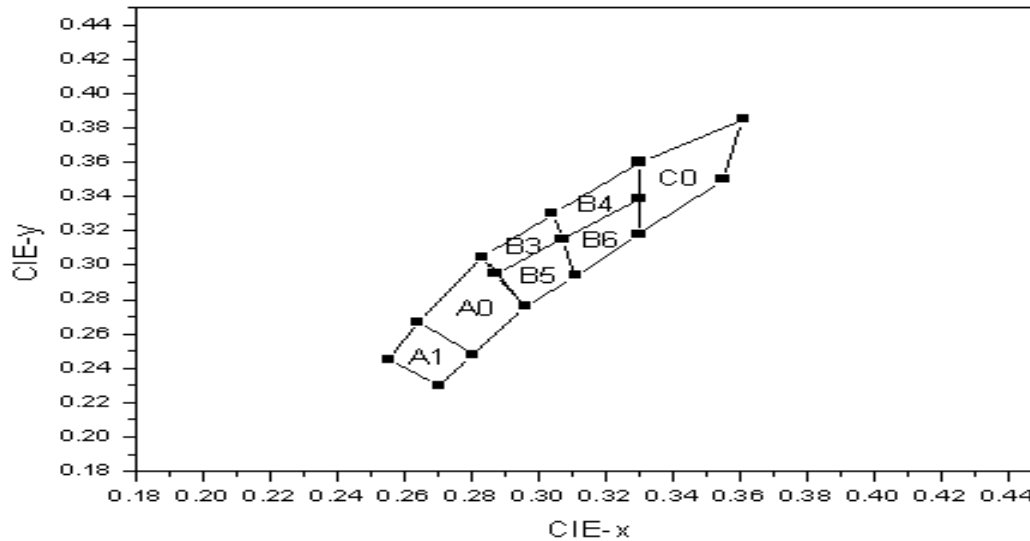
Color Ranks ( I_F=20\text{mA} , T_a=25^\circ\text{C} )
