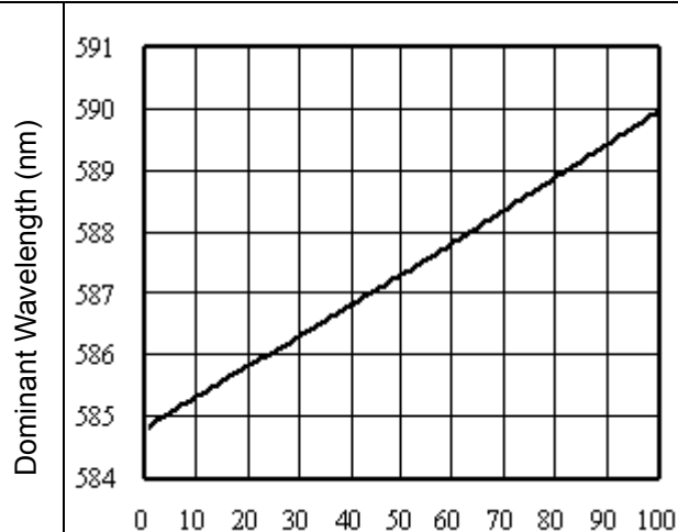
Dominant Wavelength vs. Forward Current (Ta=25°C)
