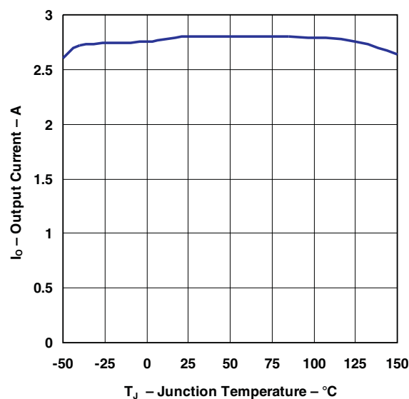
Figure 5. Current Limit
