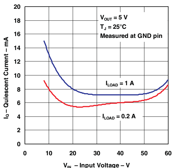
Figure 6. Quiescent Current
