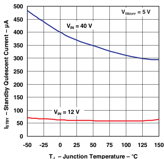
Figure 7. Standby Quiescent Current
