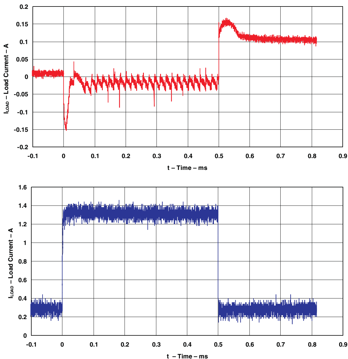
Figure 11. Load Transient Response
