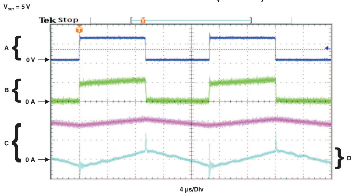
Figure 10. Switching Waveforms
