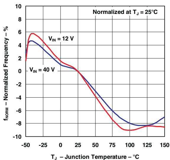
Figure 8. Oscillator Frequency
