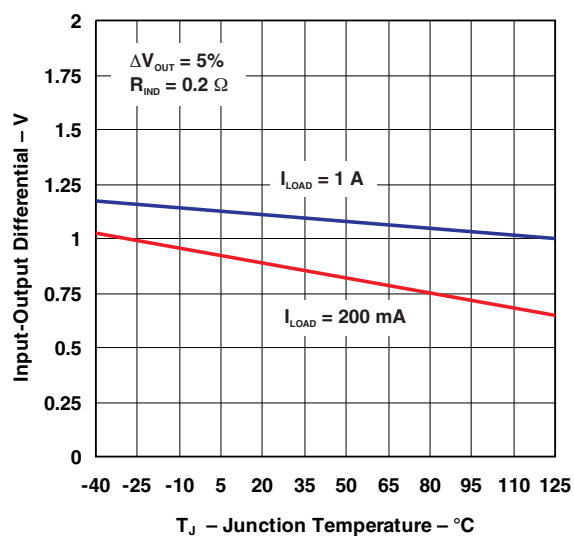
Figure 4. Dropout Voltage
