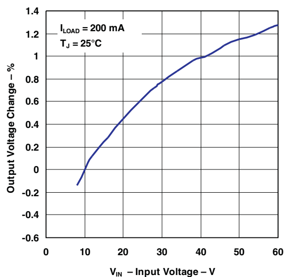
Figure 3. Line Regulation
