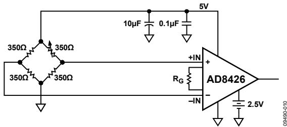
Figure 68. Precision Strain Gage
