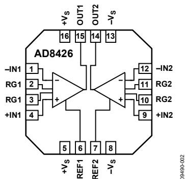
Figure 2. Pin Configuration
