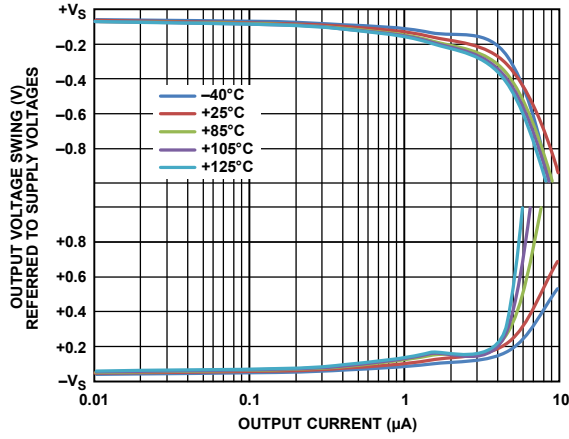
Figure 37. Output Voltage Swing vs. Output Current, G = 1
