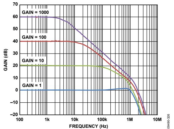
Figure 26. Gain vs. Frequency, Single Supply, V_S = 2.7\text{ V}
