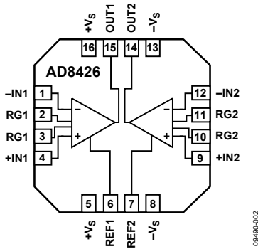
Figure 63. Pinout Diagram
