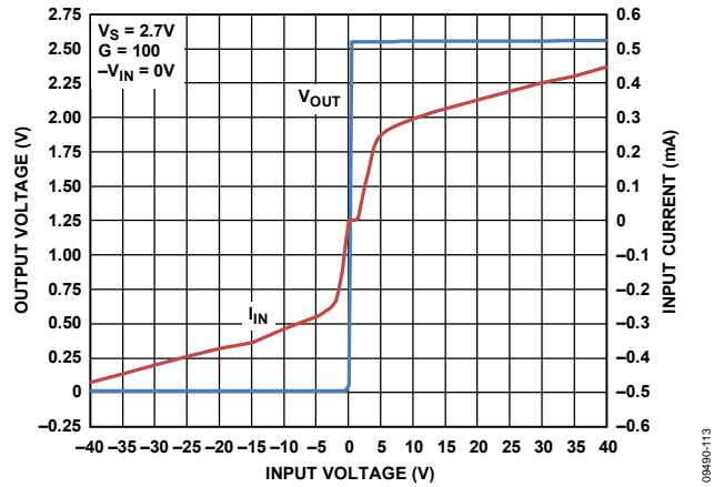
Figure 19. Input Overvoltage Performance, Single Supply, V_S = 2.7\text{ V} , G = 100
