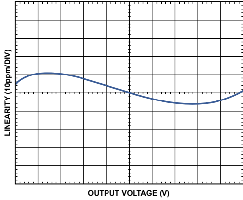
Figure 39. Gain Nonlinearity, R_L \geq 10\text{ k}\Omega , G = 10
