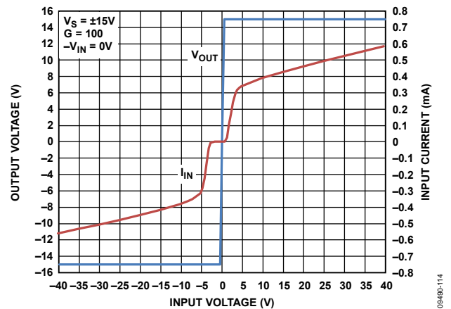
Figure 20. Input Overvoltage Performance, Dual Supply, V_S = \pm 15\text{ V} , G = 100
