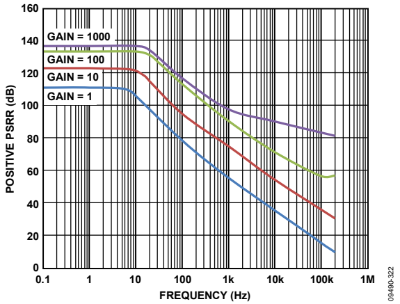
Figure 22. Positive PSRR vs. Frequency, RTI
