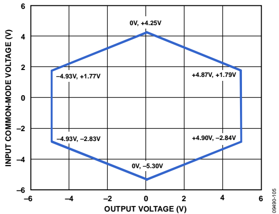
Figure 11. Input Common-Mode Voltage vs. Output Voltage, Dual Supply, V_s = \pm 5\text{ V} , G = 1
