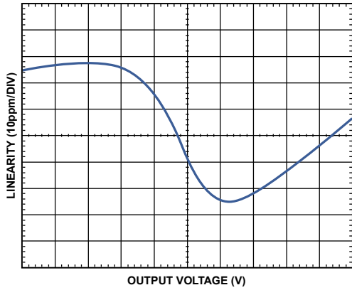
Figure 40. Gain Nonlinearity, R_L \geq 10\text{ k}\Omega , G = 100
