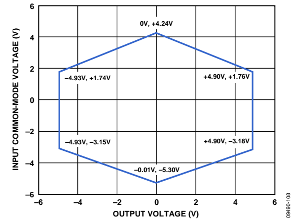
Figure 14. Input Common-Mode Voltage vs. Output Voltage, Dual Supply, V_s = \pm 5\text{ V} , G = 100
