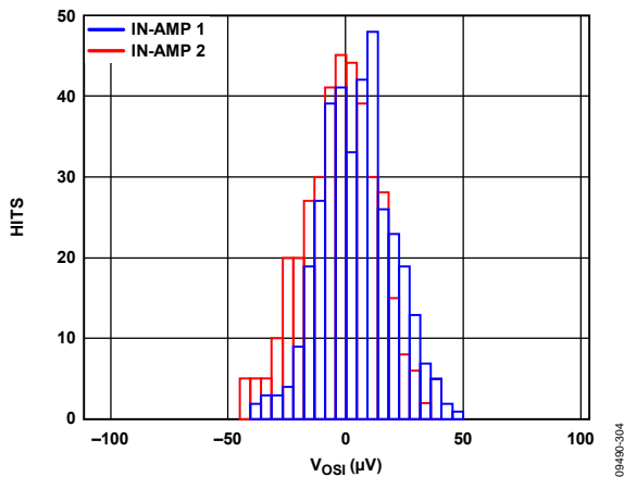
Figure 4. Typical Distribution of Input Offset Voltage
