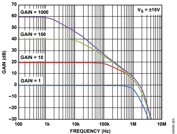
Figure 23. Gain vs. Frequency, Dual Supply, V_S = \pm 15\text{ V}
