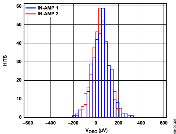
Figure 5. Typical Distribution of Output Offset Voltage
