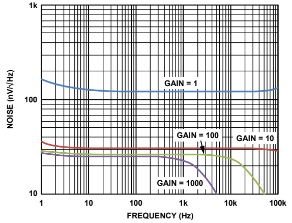
Figure 42. Voltage Noise Spectral Density vs. Frequency
