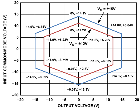
Figure 18. Input Common-Mode Voltage vs. Output Voltage, Dual Supply, V_S = \pm 15\text{ V} and V_S = \pm 12\text{ V} , G = 100
