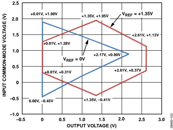
Figure 9. Input Common-Mode Voltage vs. Output Voltage, Single Supply, V_s = 2.7\text{ V} , G = 1
