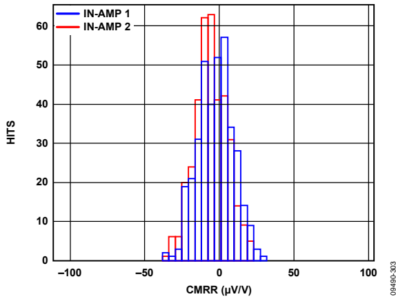
Figure 3. Typical Distribution for CMRR ( G = 1 )
