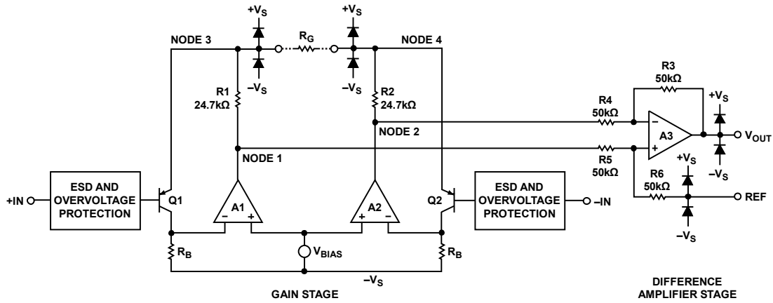
Figure 61. Simplified Schematic
