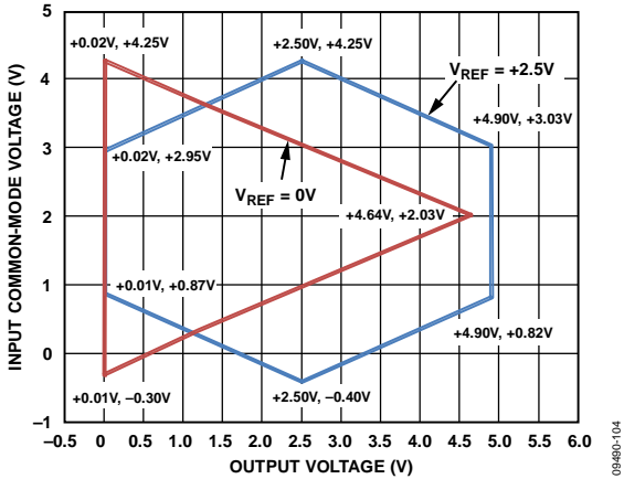
Figure 10. Input Common-Mode Voltage vs. Output Voltage, Single Supply, V_s = 5\text{ V} , G = 1
