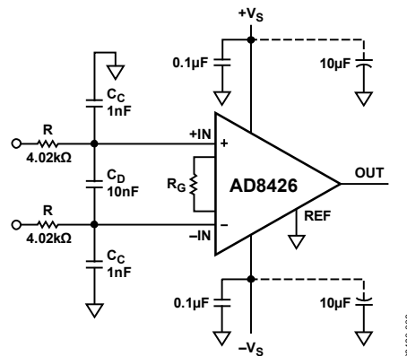
Figure 67. RFI Suppression
