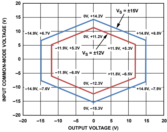
Figure 15. Input Common-Mode Voltage vs. Output Voltage, Dual Supply, V_S = \pm 15\text{ V} and V_S = \pm 12\text{ V} , G = 1
