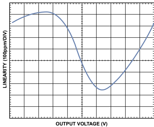
Figure 41. Gain Nonlinearity, R_L \geq 10\text{ k}\Omega , G = 1000
