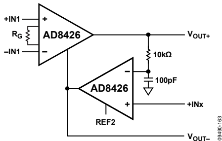
Figure 69. Differential Circuit Schematic
