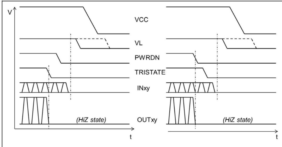
Figure 6. Power-OFF sequence
