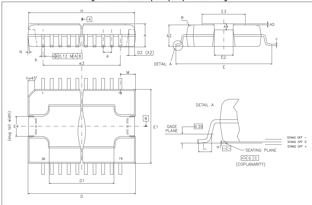
Figure 11. PowerSO36 exposed pad up outline drawing
