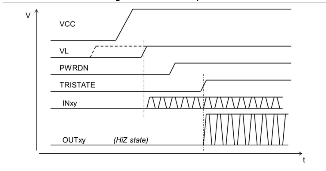
Figure 5. Power-ON sequence
