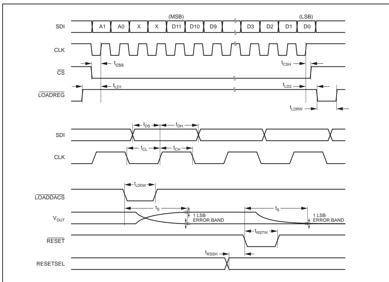
FIGURE 3. DAC7615 Timing.
