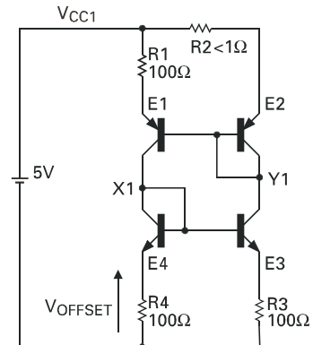
Figure 2 Output Zero-Offset Voltage Test Circuit
