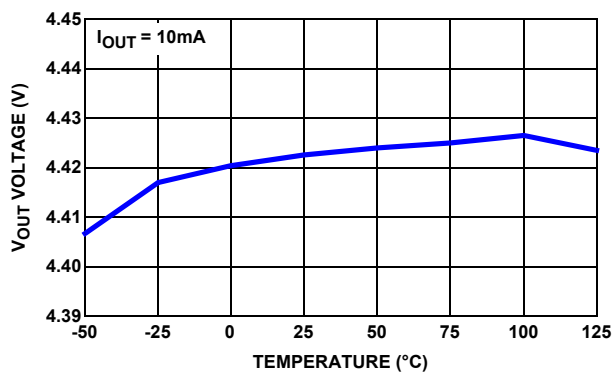
FIGURE 19. OUTPUT VOLTAGE REGULATION vs TEMPERATURE
