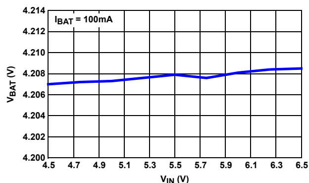
FIGURE 21. BATTERY VOLTAGE vs INPUT VOLTAGE
