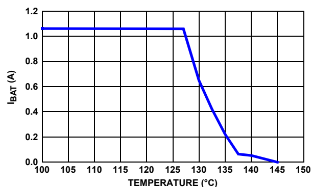
FIGURE 17. THERMAL REGULATION OF I_{BAT}
