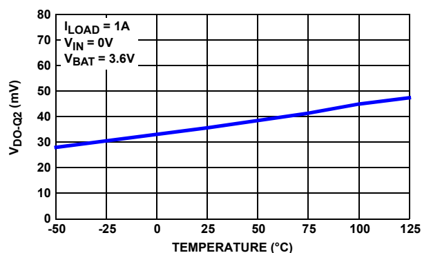
FIGURE 15. DROPOUT VOLTAGE (Q2) vs TEMPERATURE
