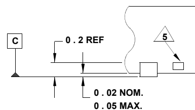
DETAIL "X"
