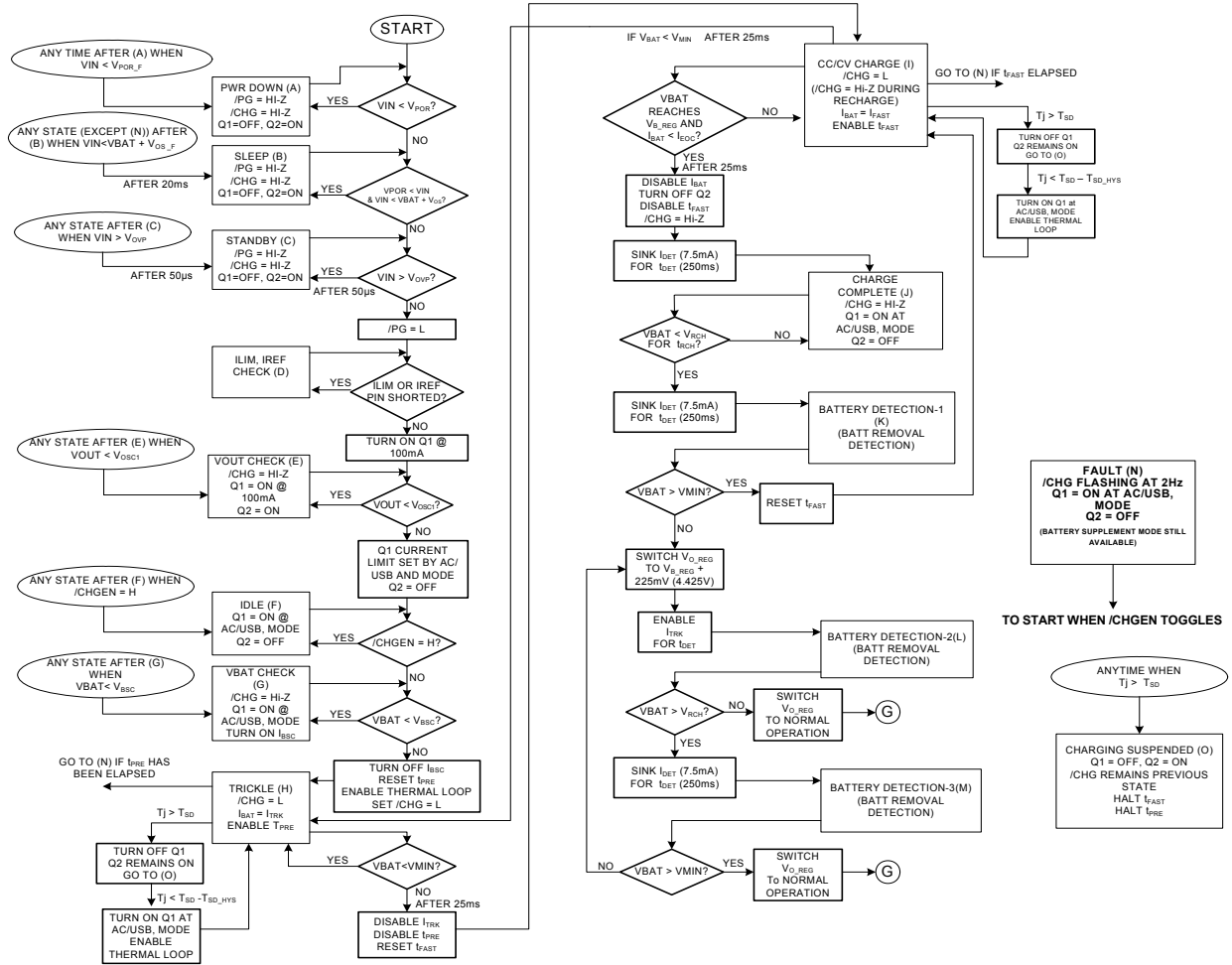
FIGURE 32. STATE DIAGRAM (CONT = L)
