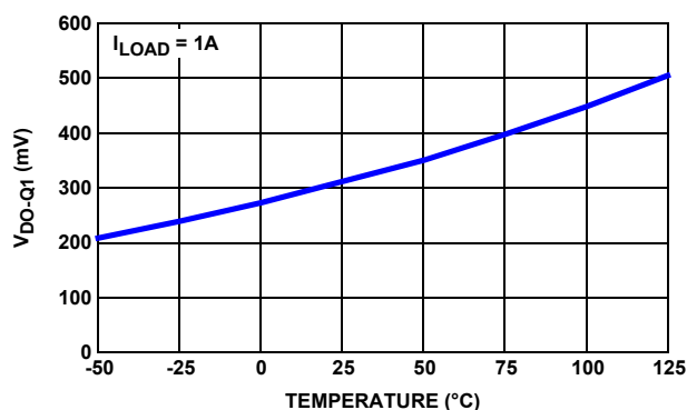
FIGURE 14. DROPOUT VOLTAGE (Q1) vs TEMPERATURE
