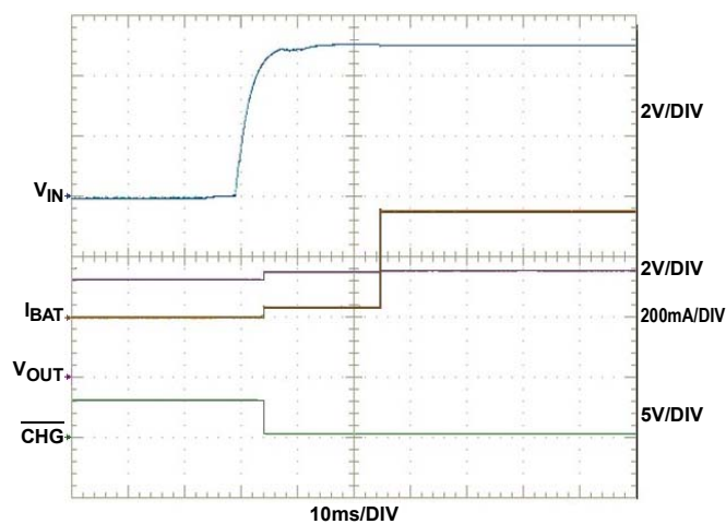
FIGURE 3. ADAPTER PLUG-IN WITH BATTERY CONNECTED
