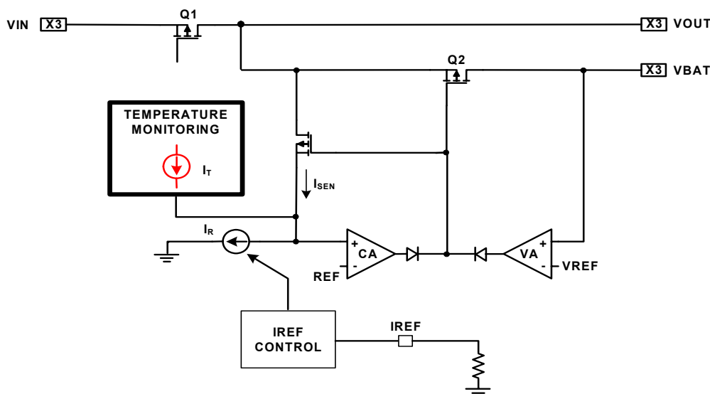
FIGURE 30. CHARGE CURRENT THERMAL FOLDBACK CONTROL
