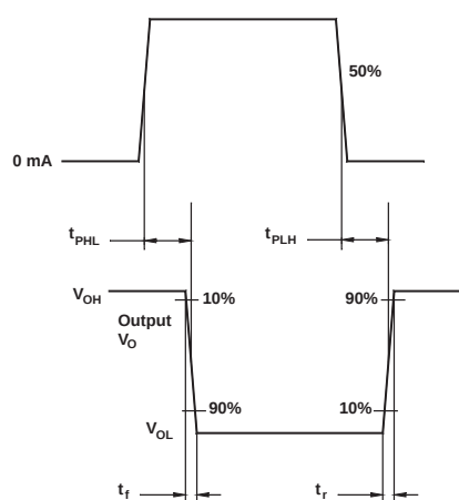
Figure 12. Switching Times Definition for Inverters
