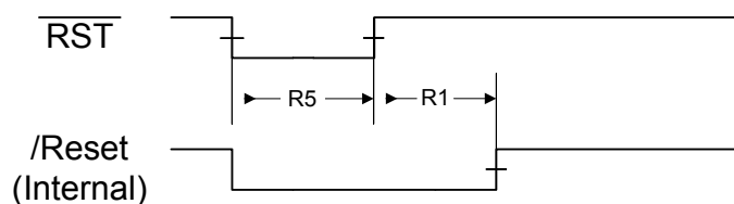
Figure 25-7. External Reset Timing ( \overline{\text{RST}} )
