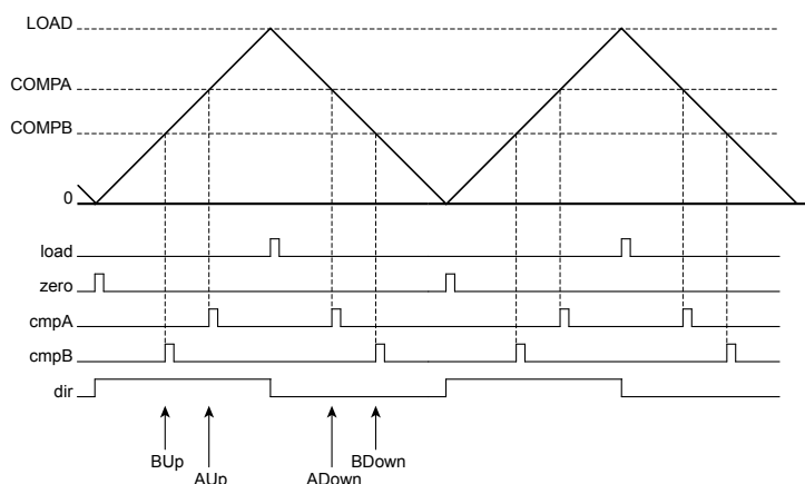
Figure 20-4. PWM Count-Up/Down Mode
