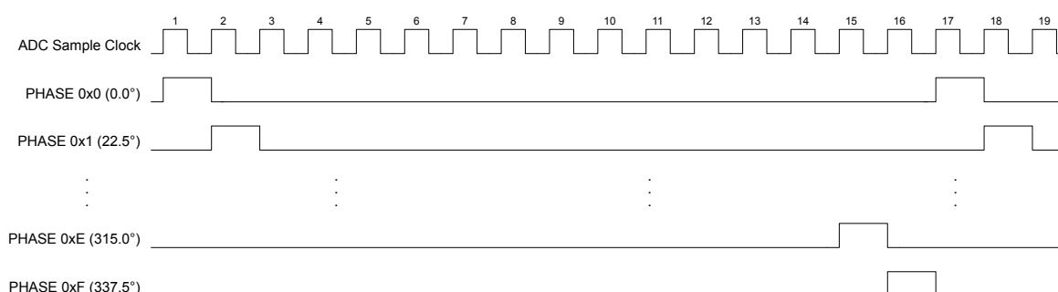
Figure 13-3. ADC Sample Phases
