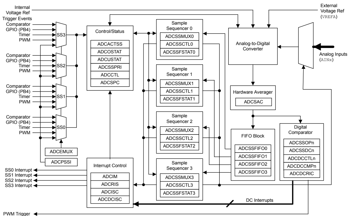
Figure 13-2. ADC Module Block Diagram
