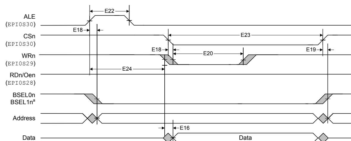
Figure 25-17. Host-Bus 8/16 Mode Write Timing
