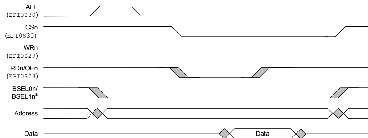
Figure 10-6. Host-Bus Read Cycle, MODE = 0x1, WRHIGH = 0, RDHIGH = 0
