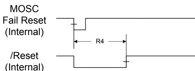
Figure 25-10. MOSC Failure Reset Timing
