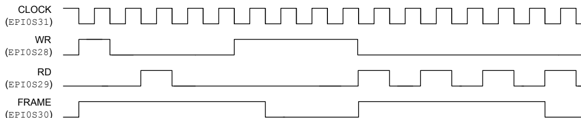
Figure 10-21. FRAME Signal Operation, FRM50=1 and FRMCNT=2
