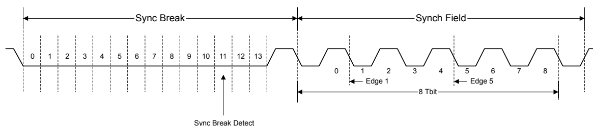
Figure 14-5. LIN Synchronization Field
