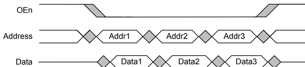
Figure 10-10. Continuous Read Mode Accesses
