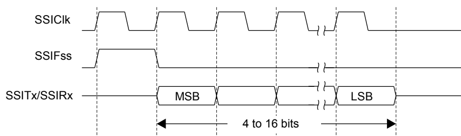
Figure 15-2. TI Synchronous Serial Frame Format (Single Transfer)
