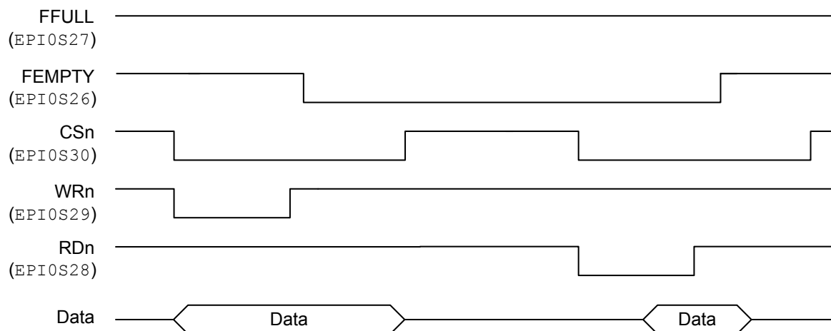
Figure 10-12. Two-Entry FIFO
