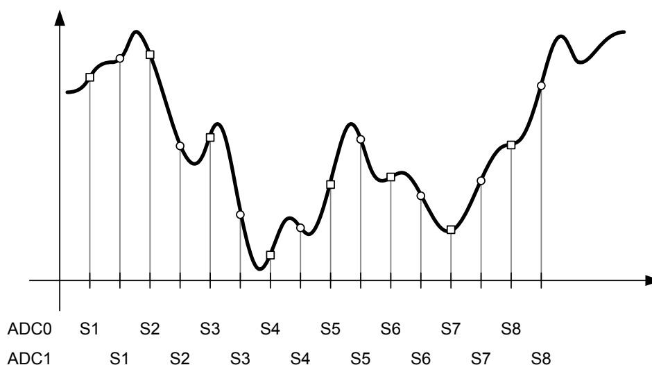
Figure 13-5. Skewed Sampling
