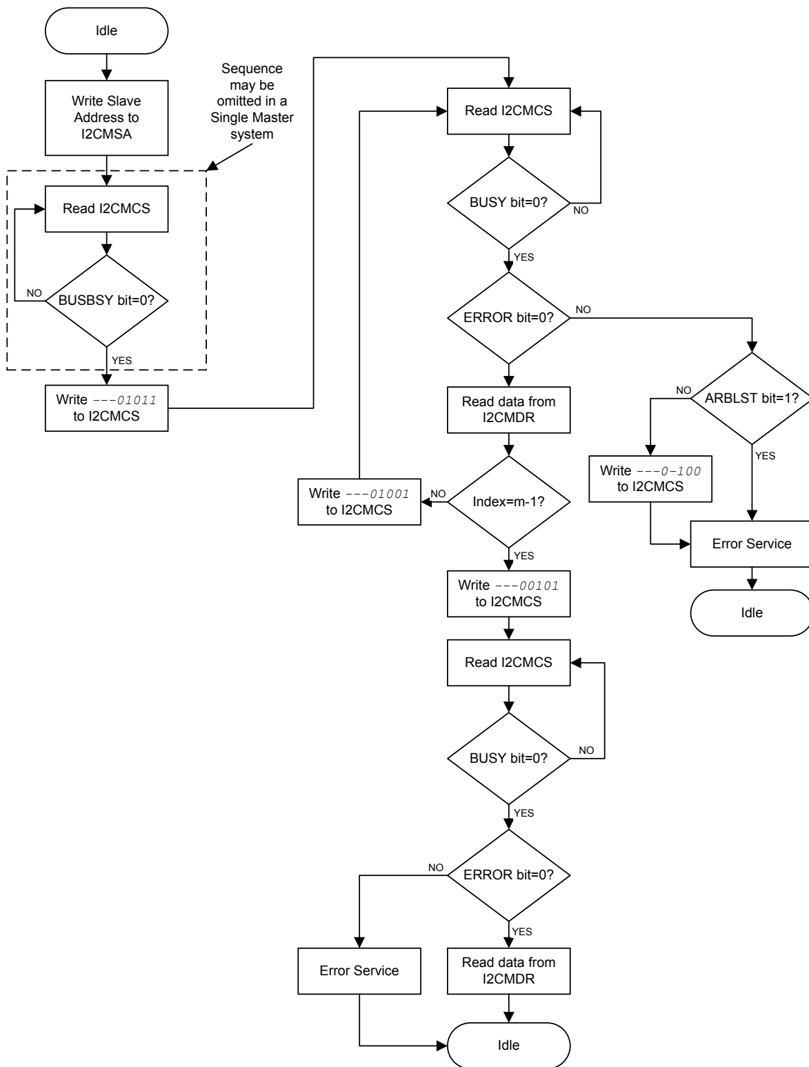
Figure 16-10. Master RECEIVE with Repeated START
