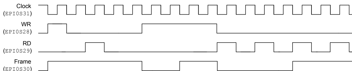
Figure 10-20. FRAME Signal Operation, FRM50=1 and FRMCNT=1
