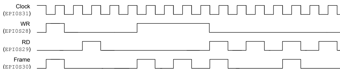
Figure 10-17. FRAME Signal Operation, FRM50=0 and FRMCNT=1
