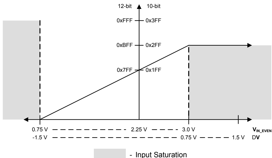
Figure 13-13. Differential Sampling Range, V_{IN\_ODD} = 2.25\text{ V}
