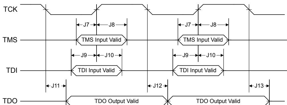
Figure 25-3. JTAG Test Access Port (TAP) Timing
