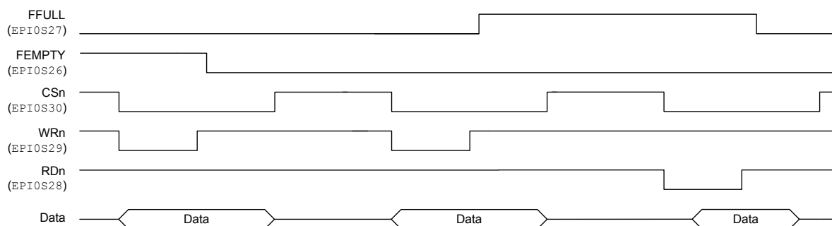
Figure 10-12. Two-Entry FIFO
