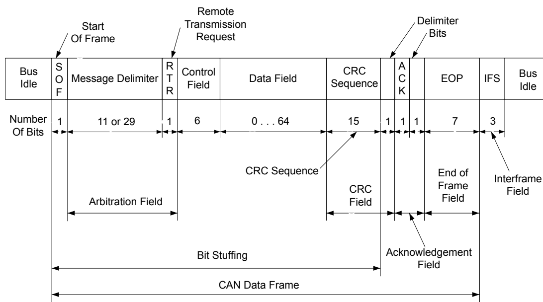
Figure 17-2. CAN Data/Remote Frame
