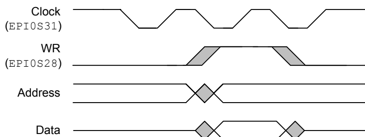
Figure 10-24. EPI Clock Operation, CLKGATE=1, WR2CYC=1
