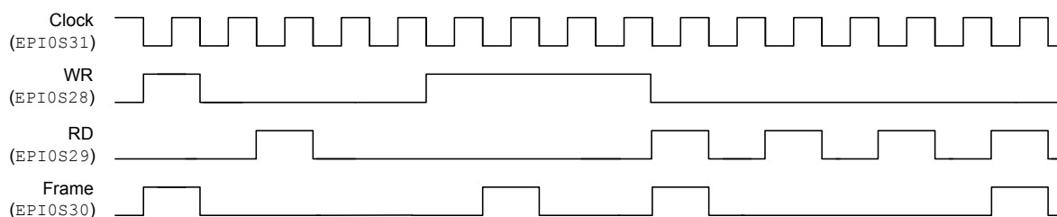
Figure 10-18. FRAME Signal Operation, FRM50=0 and FRMCNT=2
