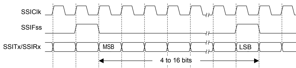
Figure 15-3. TI Synchronous Serial Frame Format (Continuous Transfer)
