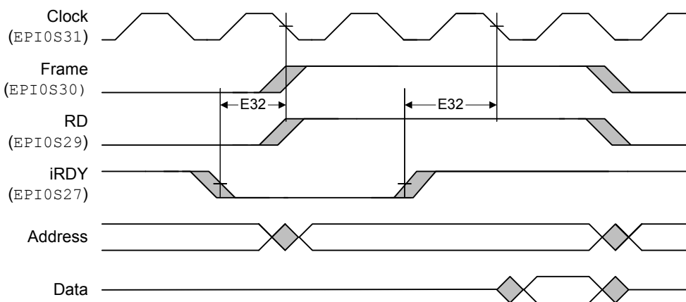
Figure 25-21. General-Purpose Mode iRDY Timing
