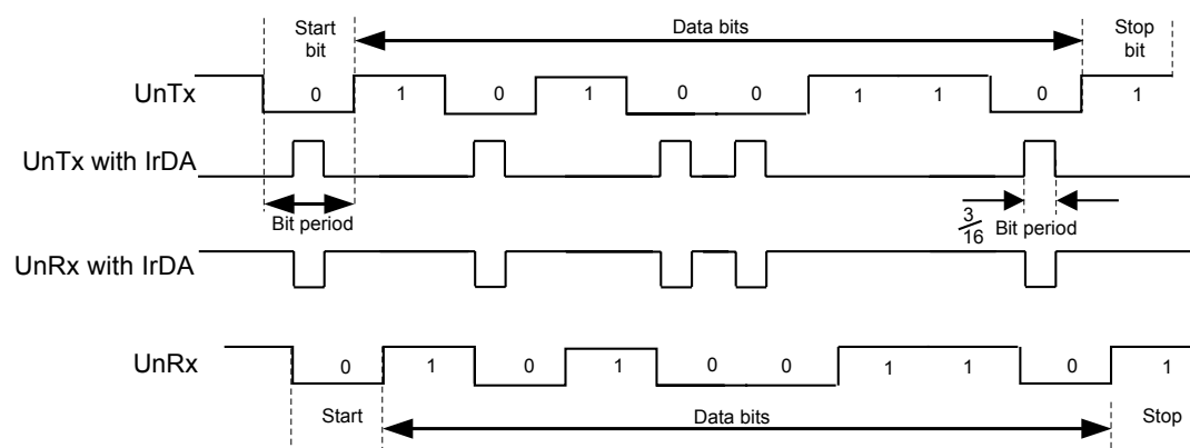
Figure 14-3. IrDA Data Modulation
