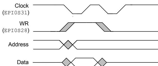
Figure 10-24. EPI Clock Operation, CLKGATE=1, WR2CYC=1
