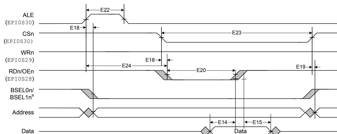
Figure 25-16. Host-Bus 8/16 Mode Read Timing
