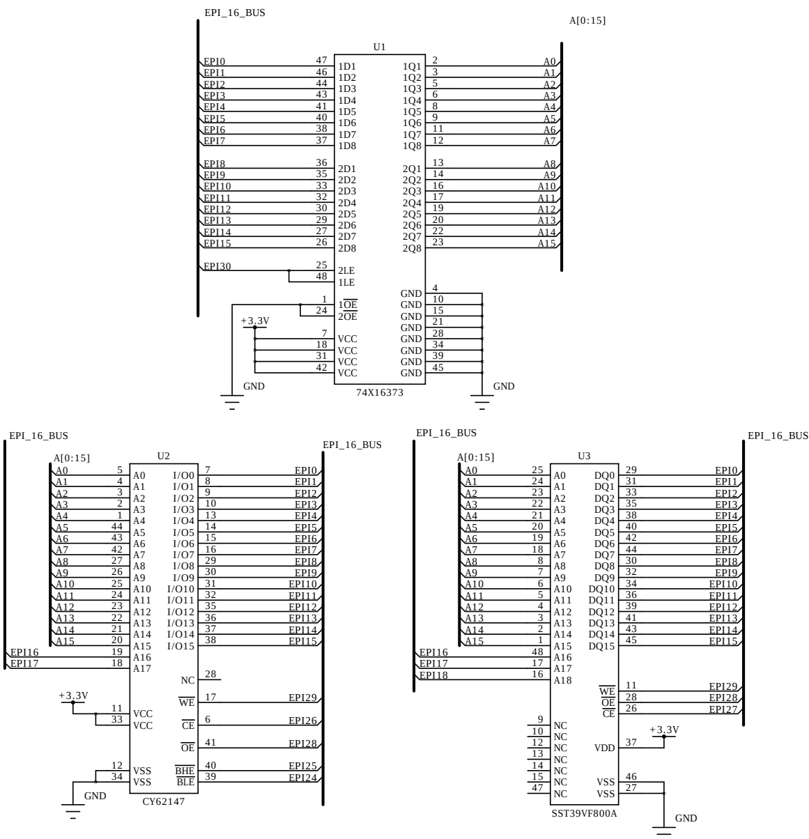
Figure 10-5. Example Schematic for Muxed Host-Bus 16 Mode
