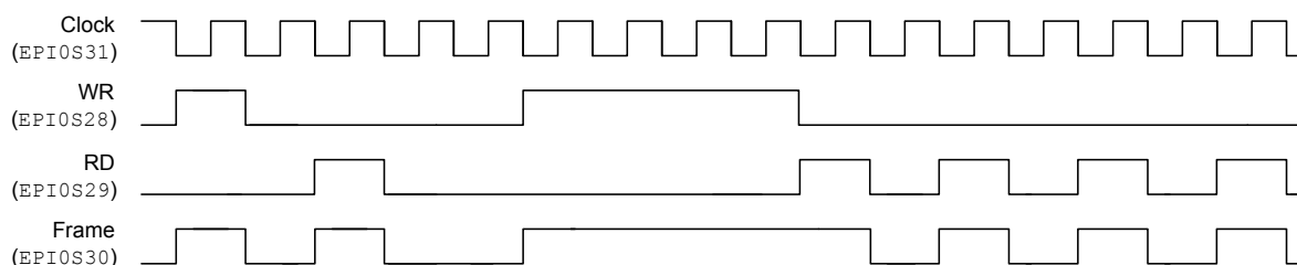
Figure 10-16. FRAME Signal Operation, FRM50=0 and FRMCNT=0
