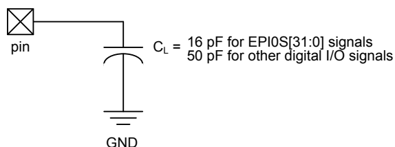
Figure 25-1. Load Conditions
