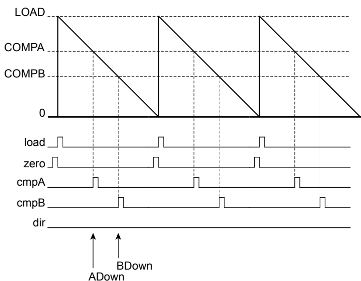
Figure 20-3. PWM Count-Down Mode
