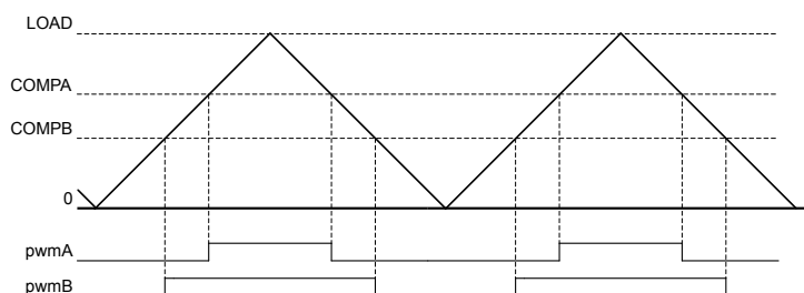
Figure 20-5. PWM Generation Example In Count-Up/Down Mode
