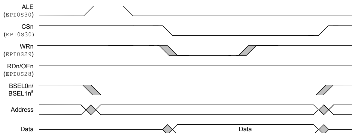
Figure 10-7. Host-Bus Write Cycle, MODE = 0x1, WRHIGH = 0, RDHIGH = 0
