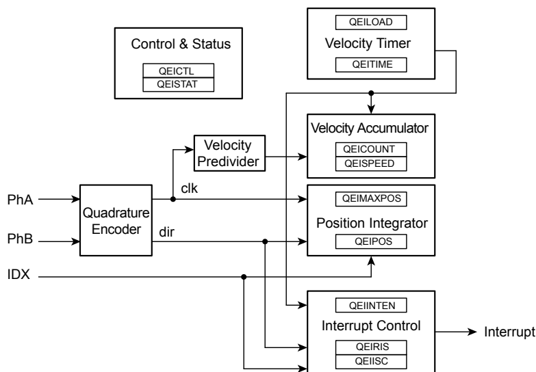
Figure 21-1. QEI Block Diagram
