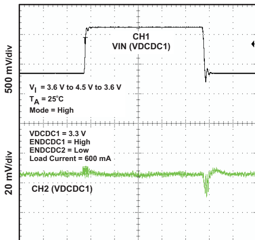
DCDC1 LINE TRANSIENT RESPONSE
