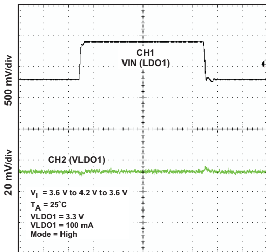
LDO1 LINE TRANSIENT RESPONSE
