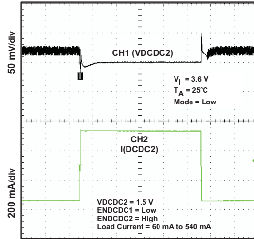
DCDC2 LOAD TRANSIENT RESPONSE
