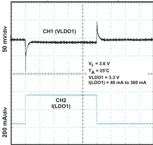
LDO1 LOAD TRANSIENT RESPONSE
