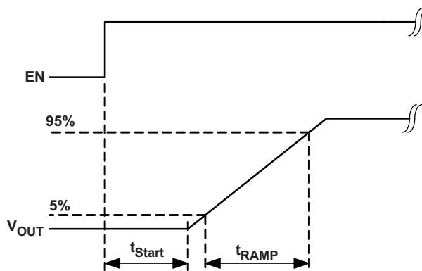
Figure 20. Soft Start
