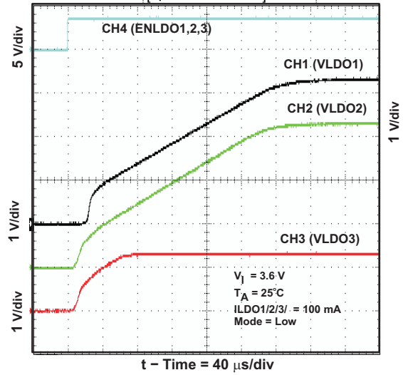
LDO1 TO LDO3 STARTUP TIMING
