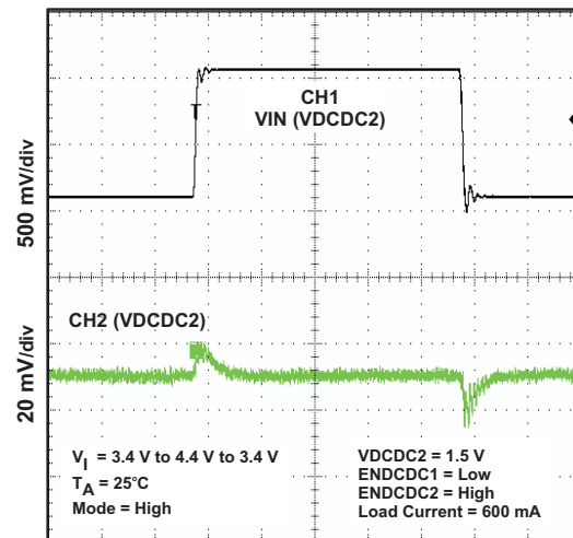
DCDC2 LINE TRANSIENT RESPONSE
