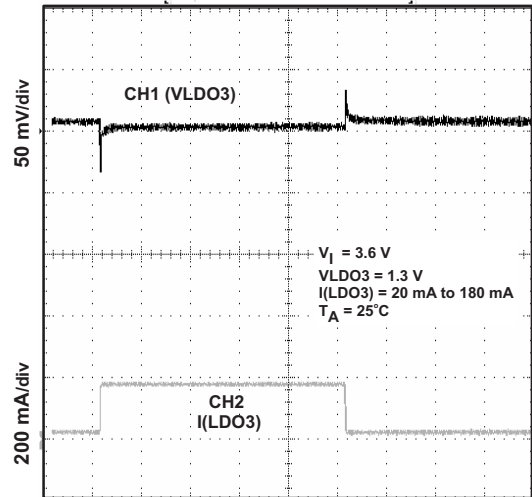
LDO3 LOAD TRANSIENT RESPONSE
