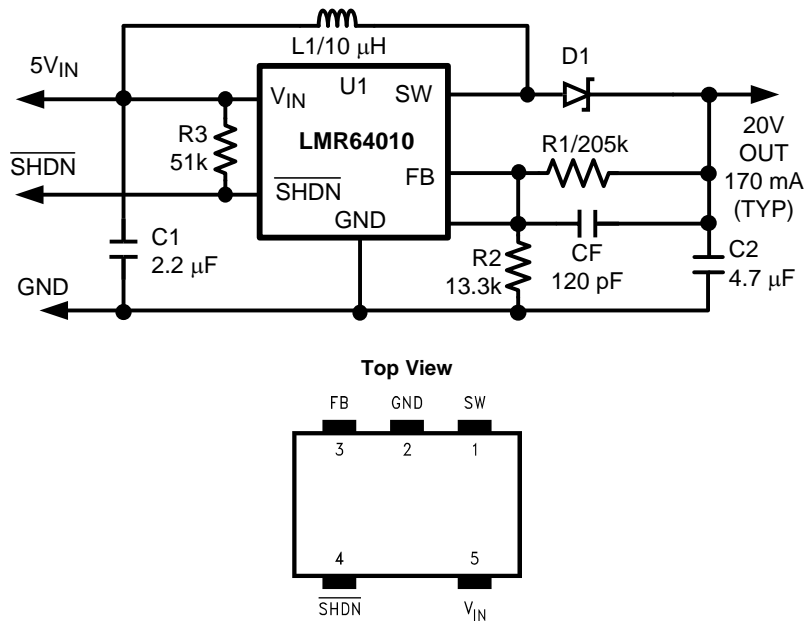
Figure 1. 5-Lead SOT-23 Package See Package Number DBV0005A
