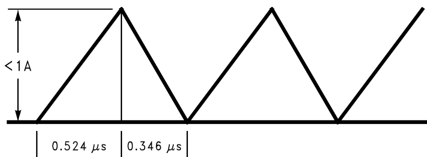
Figure 22. Discontinuous Design, 5V–12V Boost
