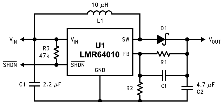
Figure 17. Basic Application Circuit
