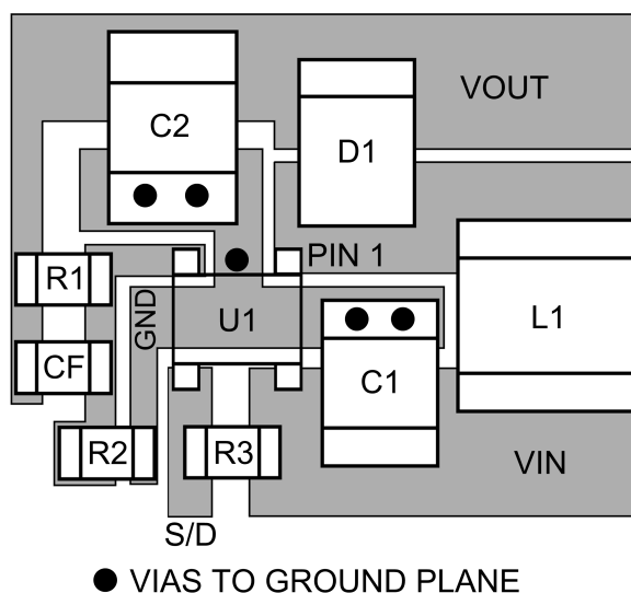
Figure 16. Recommended PCB Component Layout
