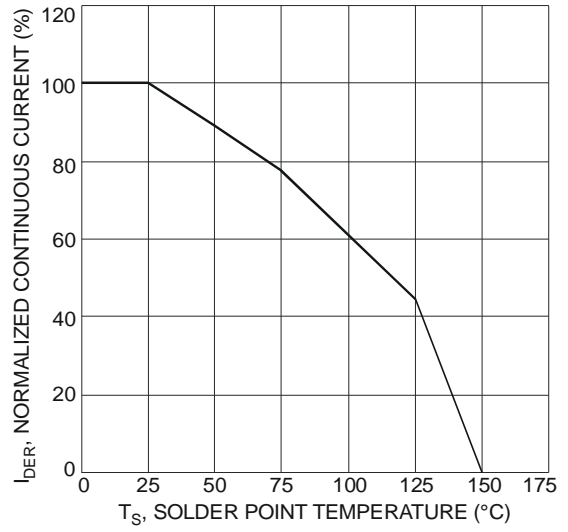
Fig 2. Normalized Continuous Current vs. Solder Point Temperature
