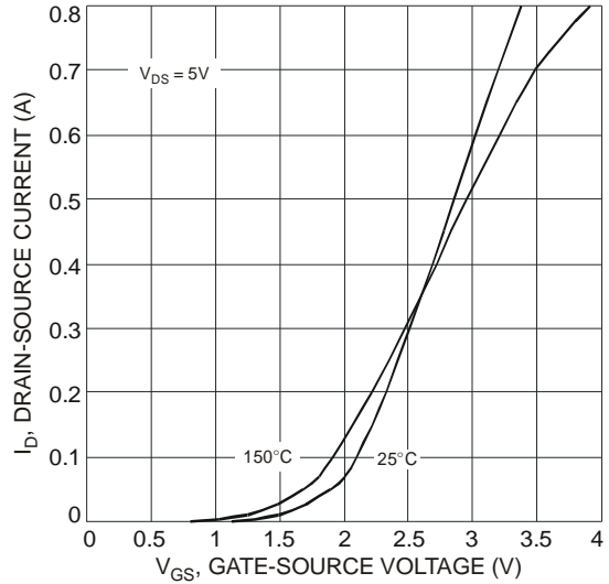
Fig. 6 Transfer Characteristics
