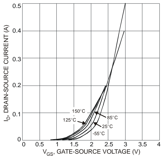
Fig. 10 Transfer Characteristics
