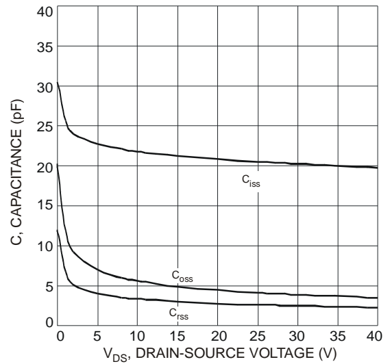
Fig. 12 Capacitance vs. Drain-Source Voltage
