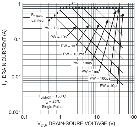
Fig 3 SOA, Safe Operation Area
