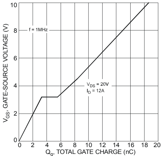
Fig. 11 Gate-Charge Characteristics
