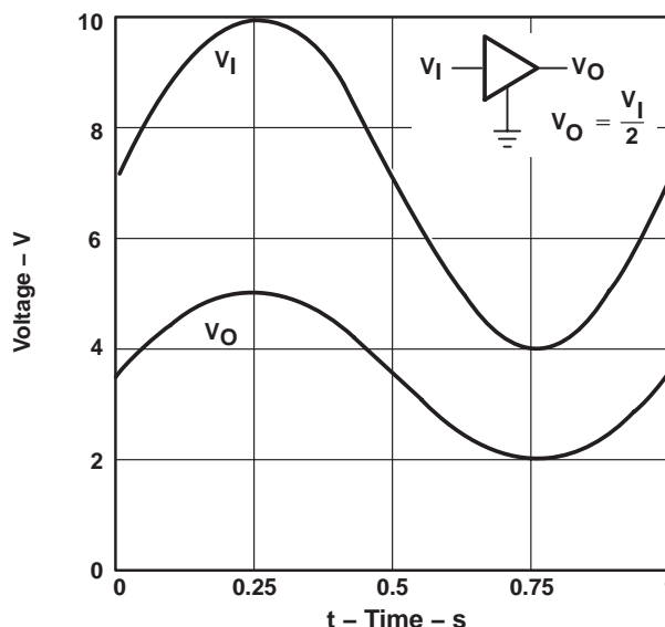
INPUT/OUTPUT TRANSFER CHARACTERISTICS
