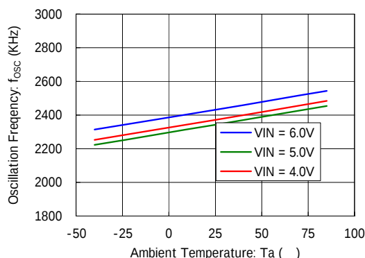
XC9242B08D
