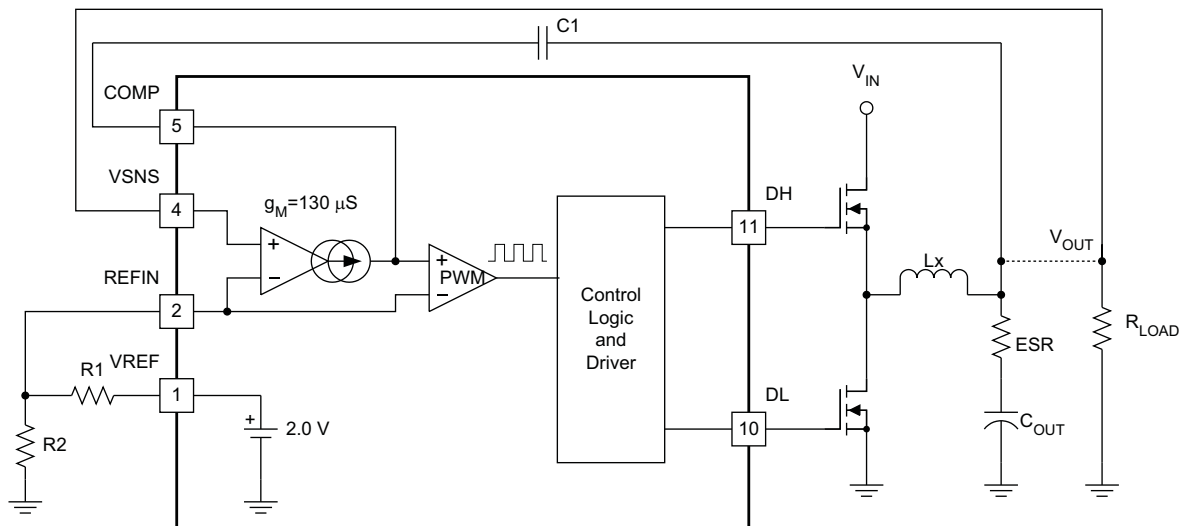
Figure 25. Simplified D-CAP™ Model
