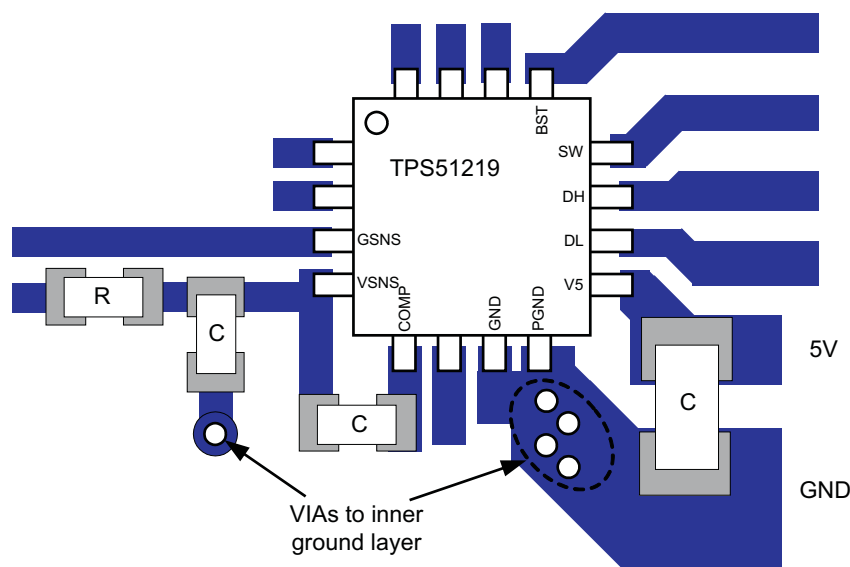
Figure 31. Case 1: COMP Pin Capacitance Connected to VSNS
