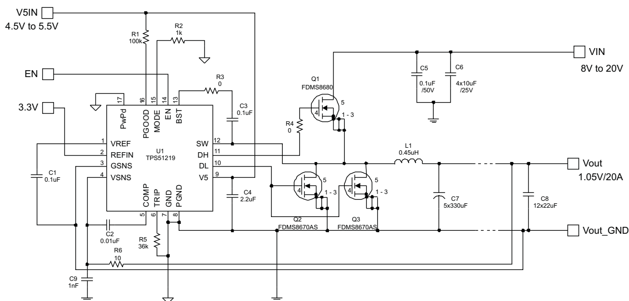
Figure 33. 1.05-V/20-A, D-CAP2™ 500-kHz, R_{DS(on)} Sensing
