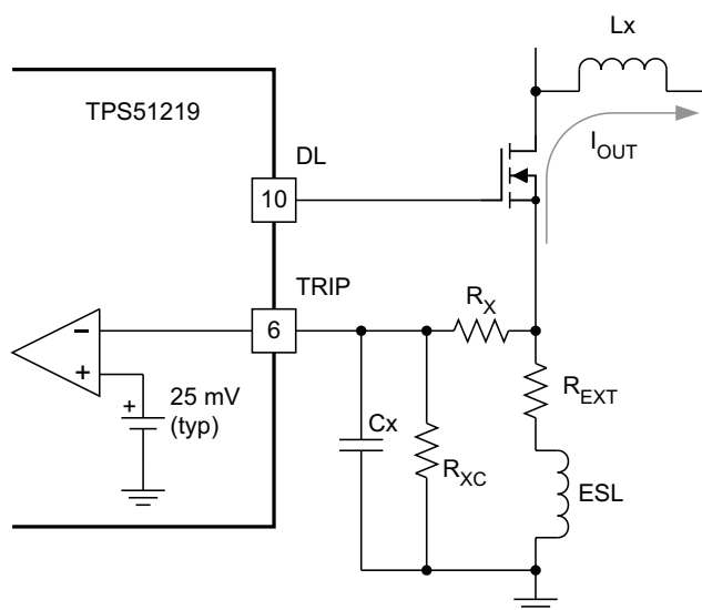
Figure 29. Adjustment of Overcurrent Limitation in Resistor Sensing
