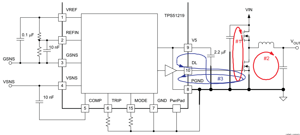
Figure 30. DC/DC Converter Ground System
