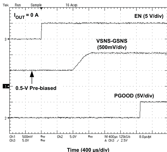
Figure 20. 1.05-V Startup Waveforms (0.5-V Pre-Biased)
