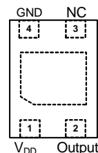
DFN1216-4
