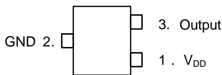
SC59
