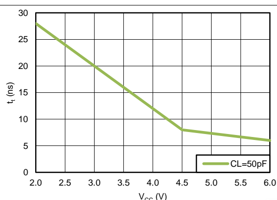
Figure 2. Transition Time vs V_{CC}
