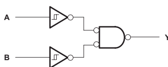
Figure 4. Logic Diagram (Positive Logic)
