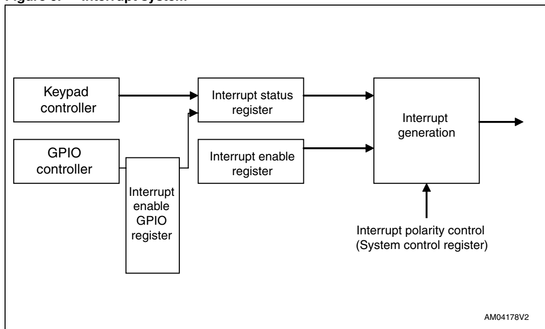
Figure 6. Interrupt system
