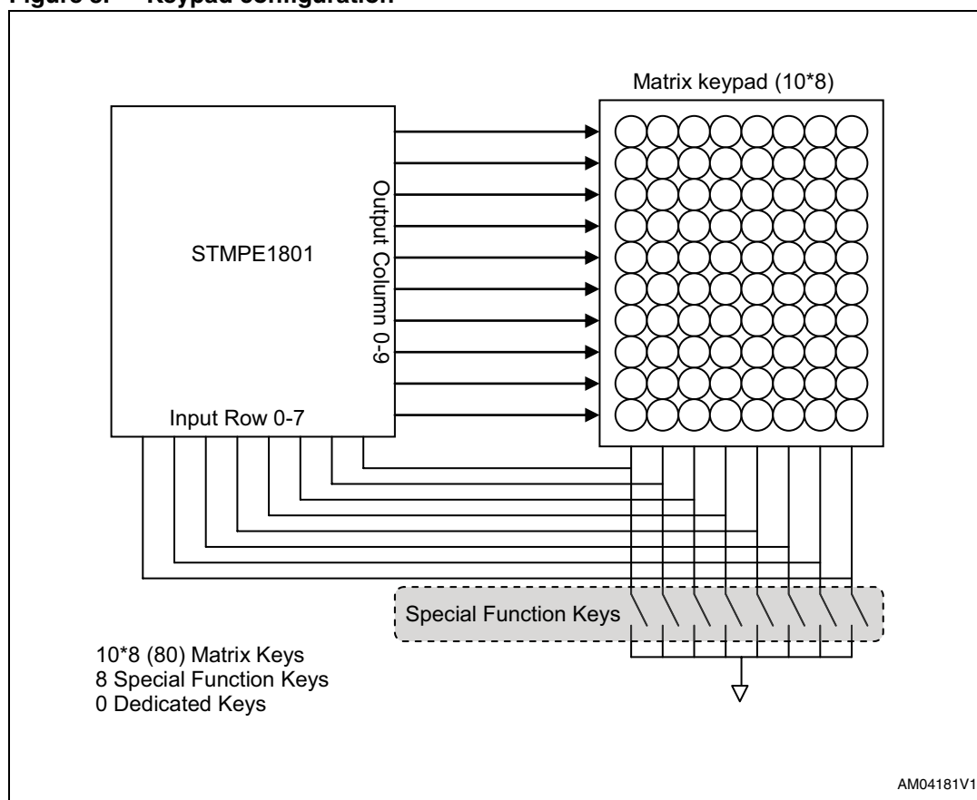
Figure 8. Keypad configuration
