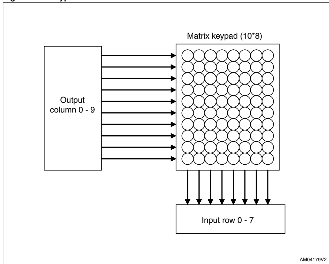
Figure 7. Keypad controller
