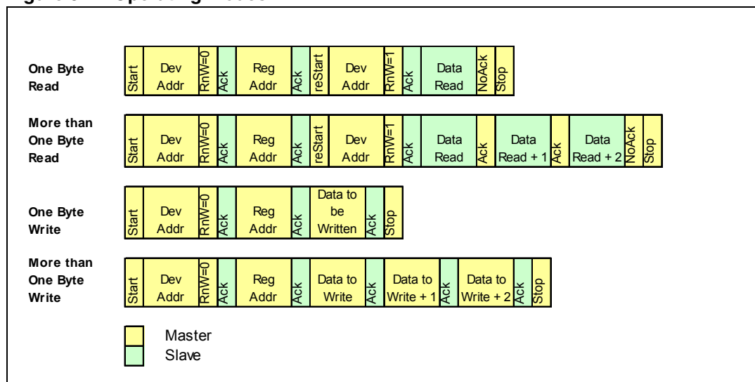
Figure 3. Operating modes
