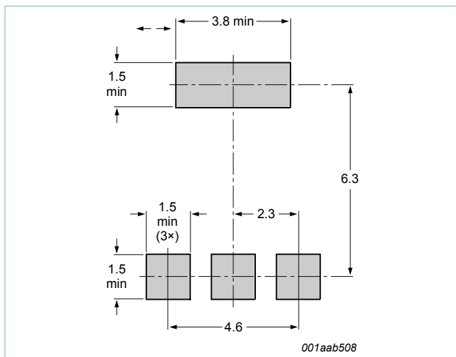
Fig. 6. Minimum footprint SOT223
