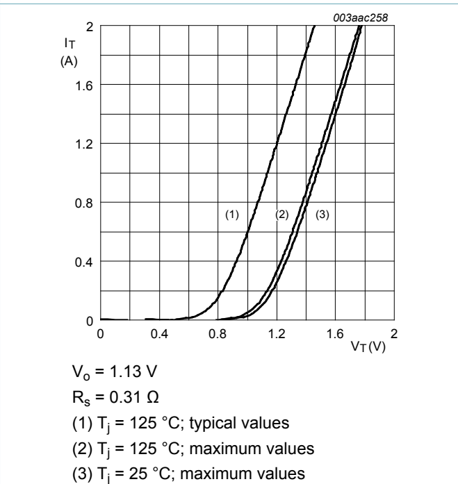
Fig. 12. On-state current as a function of on-state voltage
