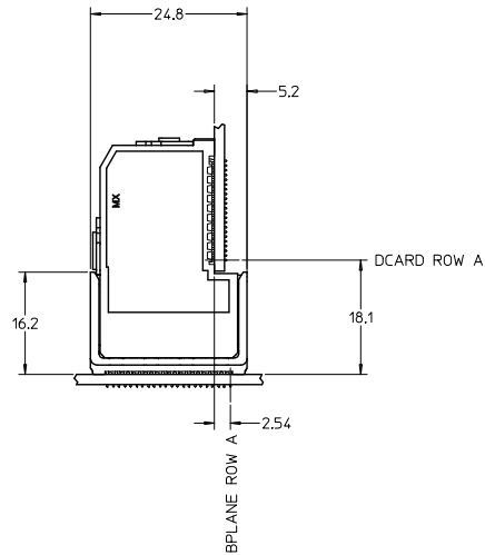
I-TRAC 11 ROW BOARD RELATIONSHIPS
