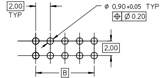
RECOMMENDED PCB PATTERN
