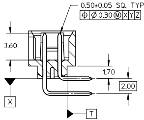
SECTION G-G
