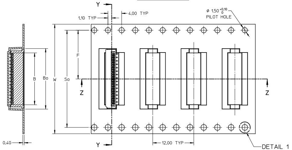
SECTION Y-Y
