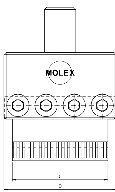
View Z
