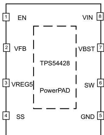
DDA Package with Thermal Pad 8-Pin SO PowerPAD Top View
