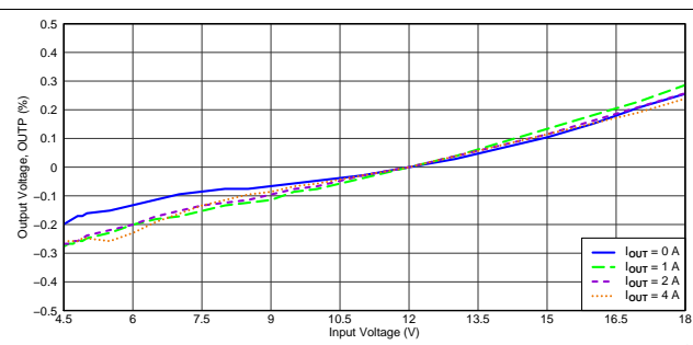
Figure 19. Line Regulation
