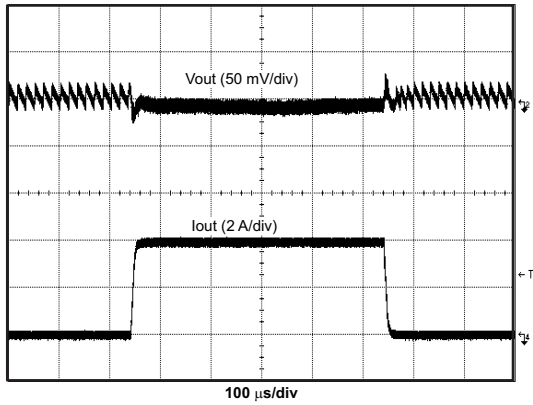
Figure 12. 1.05-V Load Transient Response
