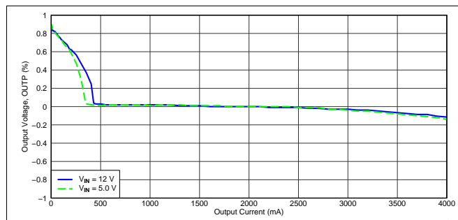
Figure 18. Load Regulation, V_{IN} = 5\text{ V} and V_{IN} = 12\text{ V}
