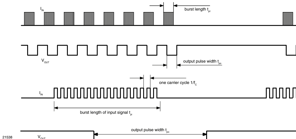
Fig. 1 - Testsignal
