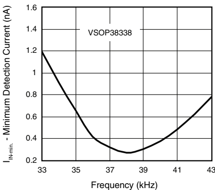
Fig. 4 - Bandpassfilter Characteristic
