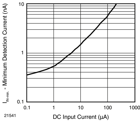
Fig. 3 - Sensitivity vs. DC Input Current
