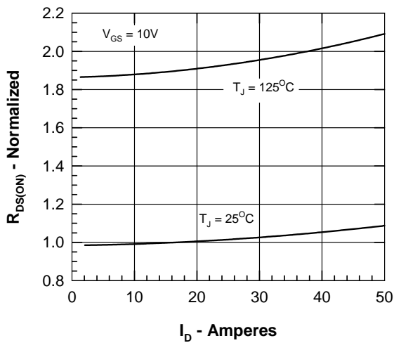
Figure 3. R_{DS(on)} normalized to 0.5 I_{D25} value vs. I_D
