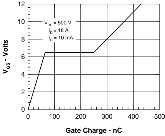
Figure 7. Gate Charge
