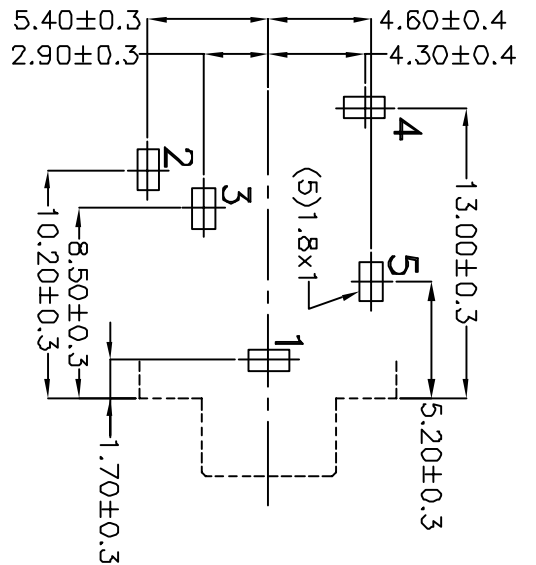
HOLE LAYOUT (TOP VIEW)
