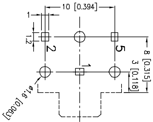
HOLE LAYOUT (TOP VIEW)
