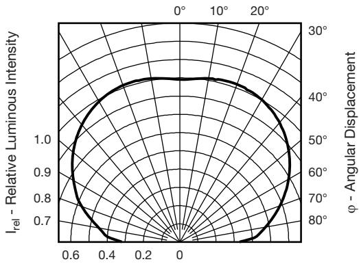
Fig. 7 - Relative Luminous Intensity vs. Angular Displacement
