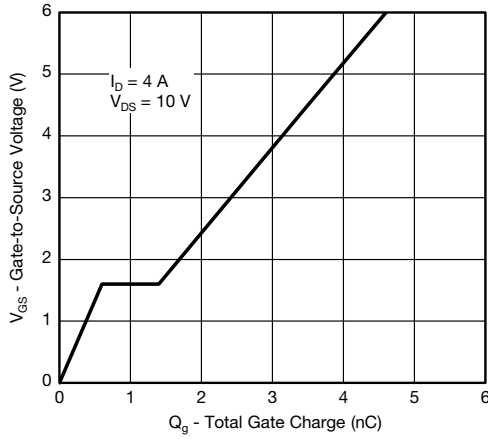
Gate Charge
