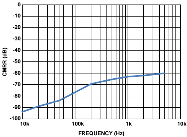
FIGURE 7. CMRR vs FREQUENCY FOR V_{DD} = 5V
