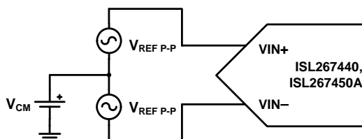
FIGURE 23. DIFFERENTIAL INPUT SIGNALING
