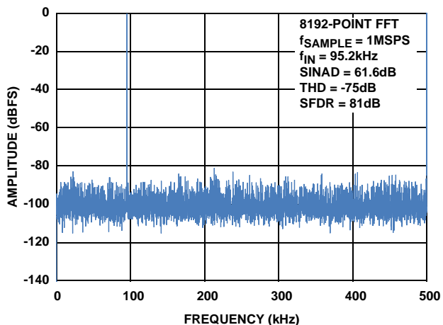
FIGURE 19. ISL267440 DYNAMIC PERFORMANCE WITH V_{DD} = 5V
