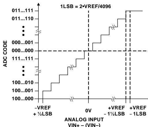
FIGURE 22. IDEAL TRANSFER CHARACTERISTICS
