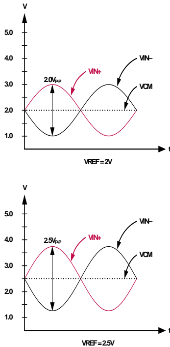
FIGURE 24. RELATIONSHIP BETWEEN VREF AND FULL-SCALE RANGE
