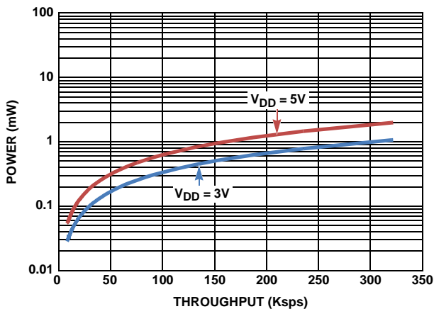
FIGURE 31. POWER CONSUMPTION vs THROUGHPUT RATE
