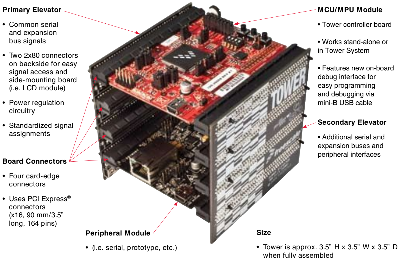
Figure 4. Freescale's Tower System
