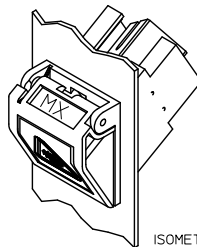
ISOMETRIC VIEW
