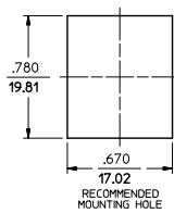
RECOMMENDED MOUNTING HOLE
