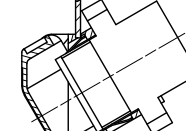
SECTION C-C VERSION 4 (MTP-MTP) SEE NOTE 2
