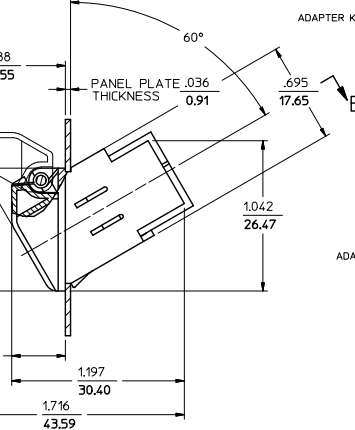
ADAPTER KEY LOCATION
