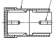
SECTION B-B VERSION 3 (SC-SC) ROTATED 30° CW
