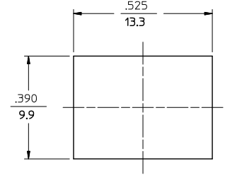
RECOMMENDED MOUNTING PATTERN FOR \frac{.063}{1.6} THICK PANEL
