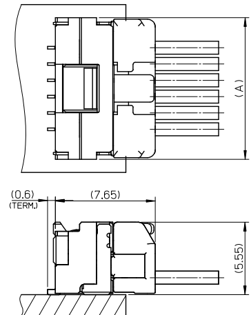
嵌合図 MATED CONNECTORS
