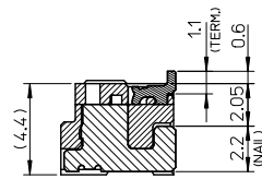
SECTION Z-Z
