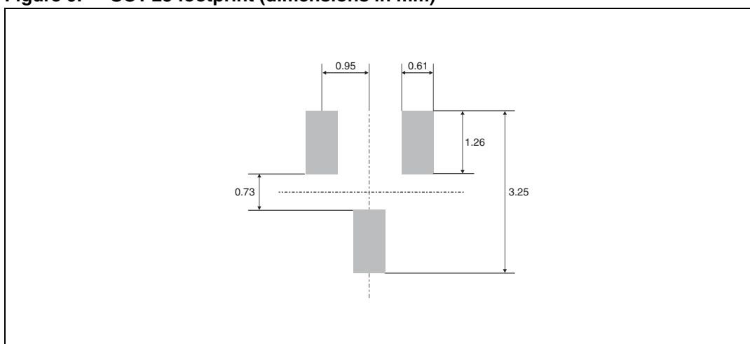
Figure 9. SOT-23 footprint (dimensions in mm)
