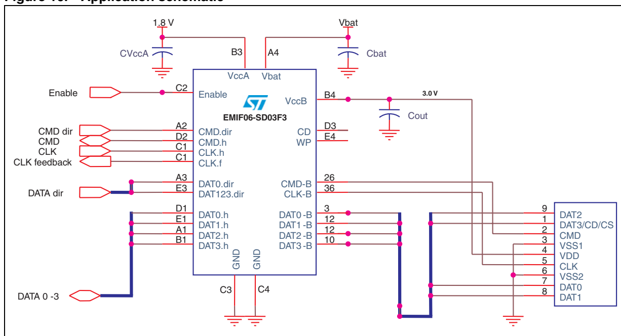
Figure 16. Application schematic
