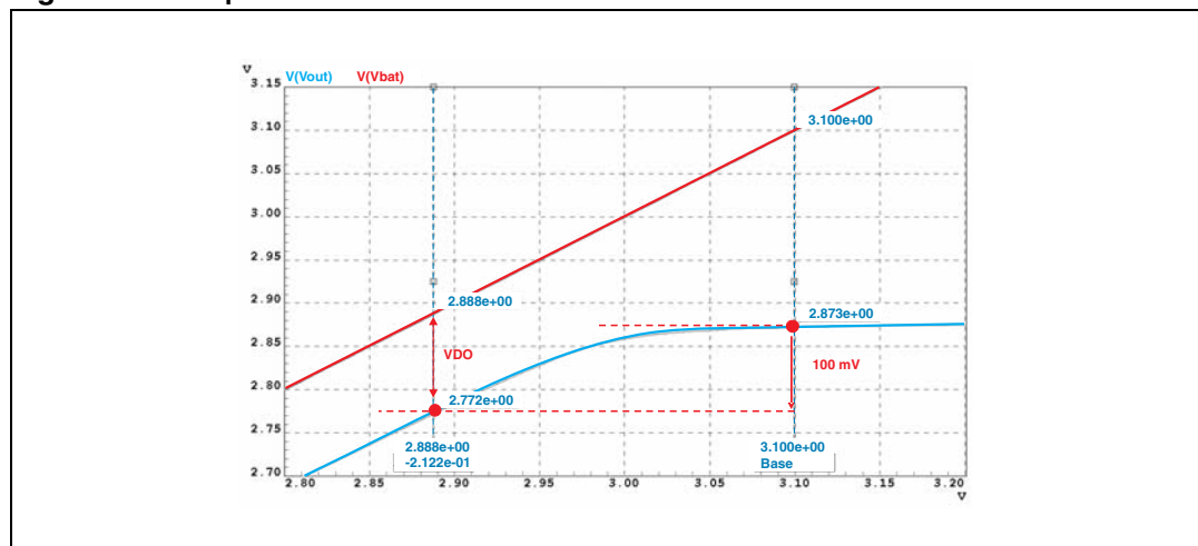
Figure 15. Dropout definition
