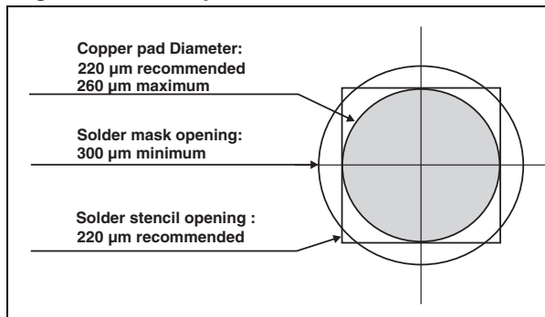
Figure 19. Footprint recommendations
