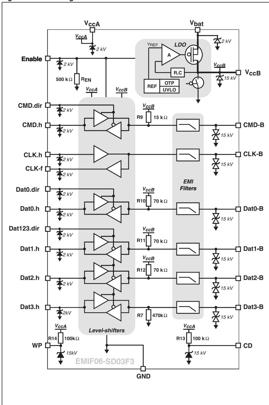
Figure 3. Block diagram
