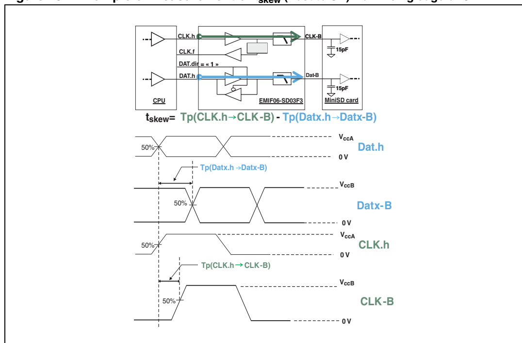
Figure 10. Example of measurement of t_{\text{skew}} (host to SD) from rising edge of CLK.h
