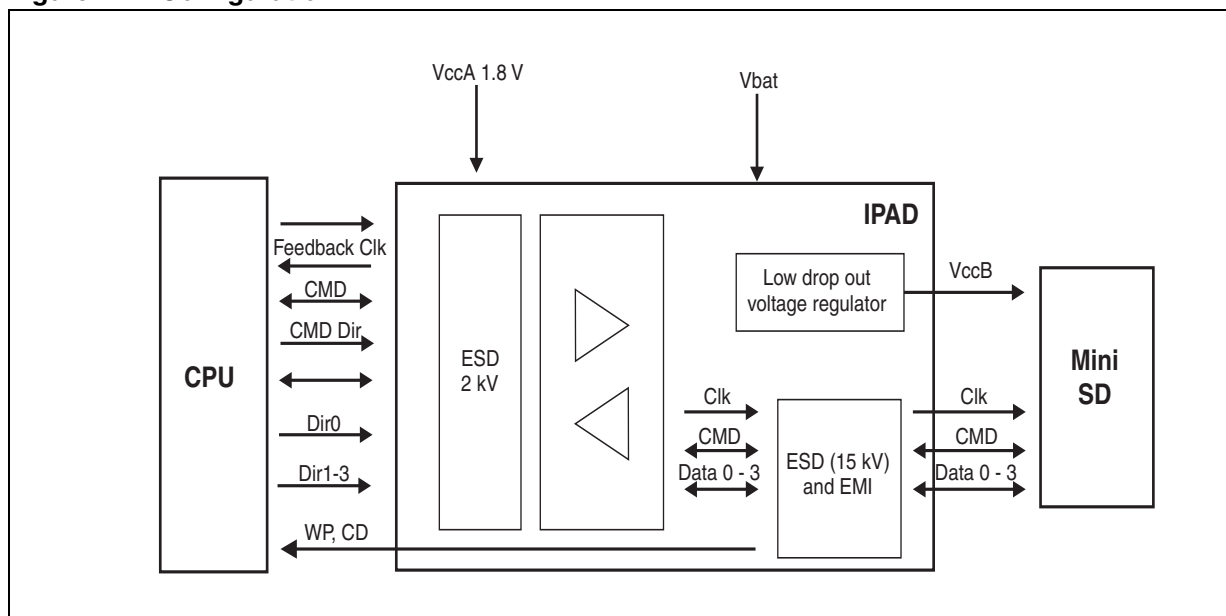
Figure 2. Configuration
