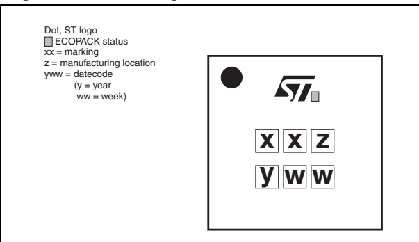
Figure 20. Marking
