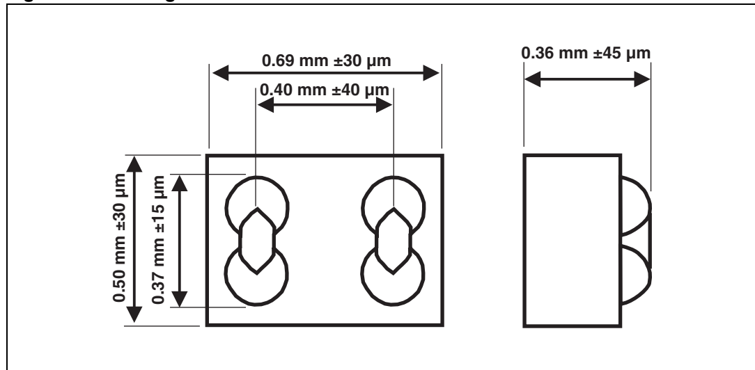
Figure 12. Package dimensions
