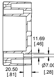
SECTION C-C MOUNTING HOLE
