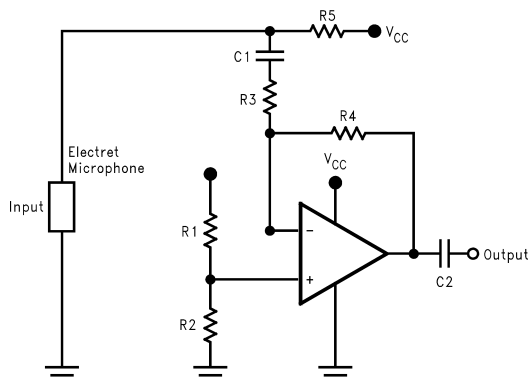
Figure 33. A Battery Powered Microphone Preamplifier
