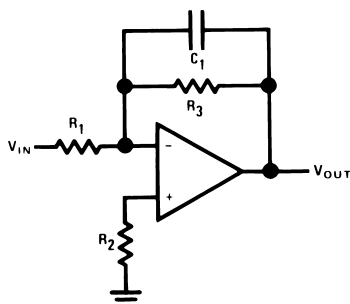
Figure 31. Simple Low-Pass Active Filter
