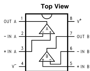
Figure 35. 8-Pin SOIC and VSSOP Packages See Package Numbers D0008A and DGK0008A
